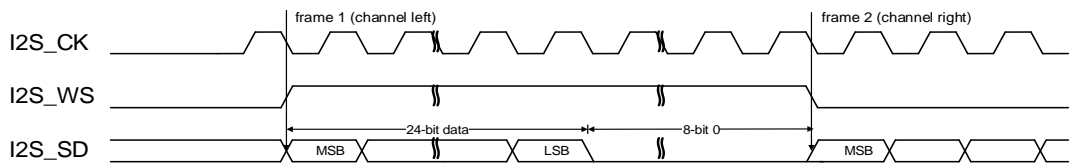
Figure 22-28. MSB justified standard timing diagram (DTLEN=01, CHLEN=1, CKPL=1)
