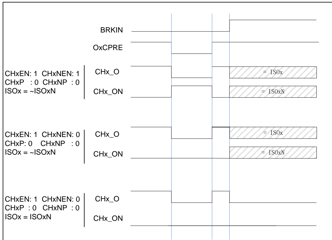
Figure 18-95. Output behavior in response to a break(The break high active)
