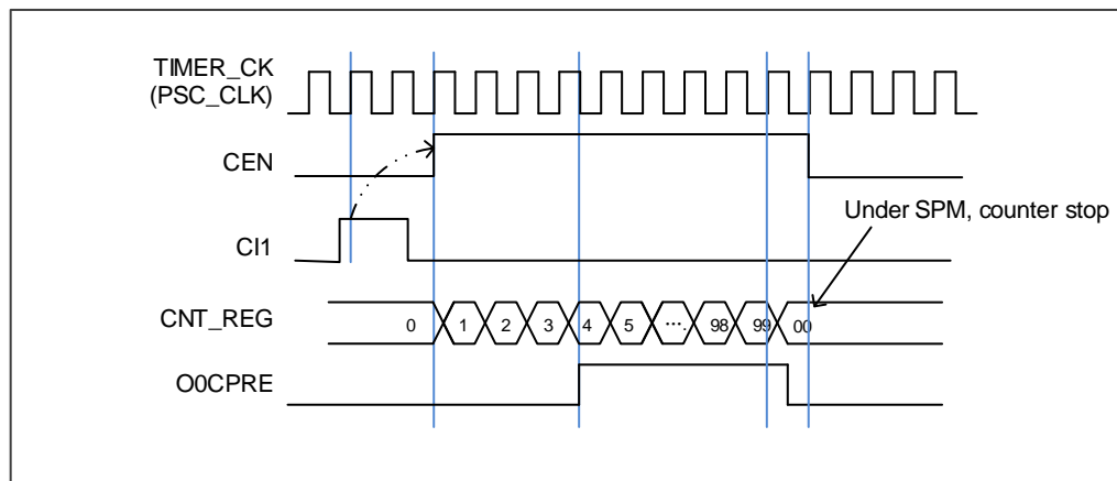
Figure 18-83. Single pulse mode TIMERx_CHxCV = 4 TIMERx_CAR=99
