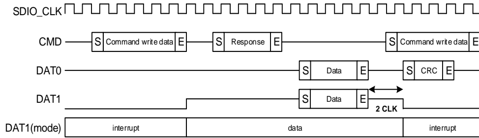
Figure 24-16. Write interrupt cycle timing
