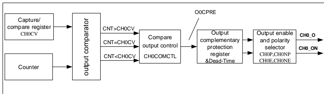
Figure 18-91. Channel output compare principle (with complementary output, x=0)
