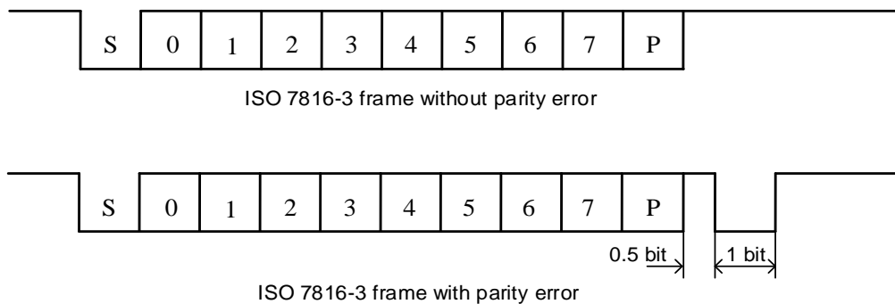
Figure 20-31. ISO7816-3 frame format
