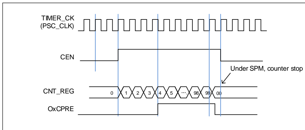
Figure 18-96. Single pulse mode TIMERx_CHxCV = 0x04 TIMERx_CAR=0x60
