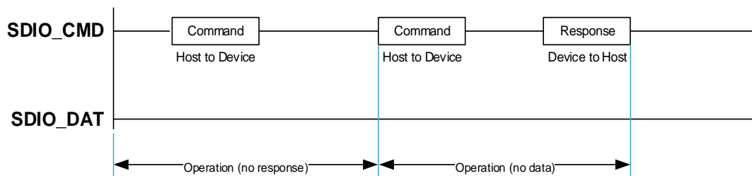
Figure 24-1. SDIO “no response” and “no data” operations
