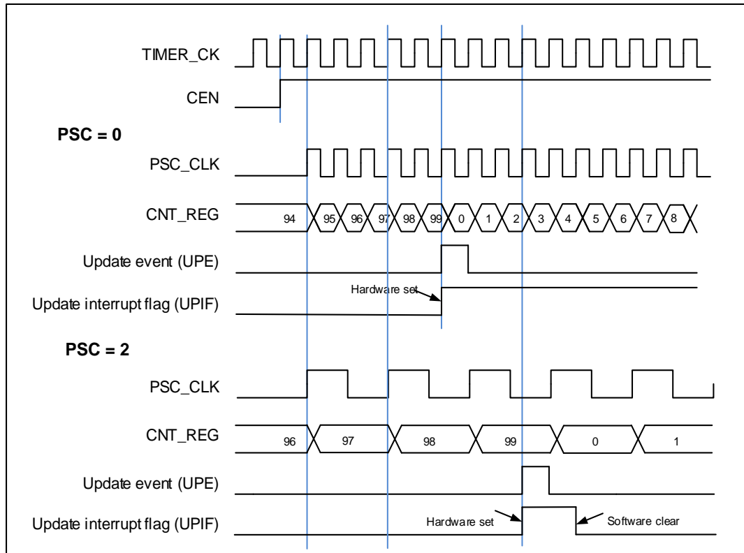
Figure 18-100. Timing chart of up counting mode, PSC=0/2
