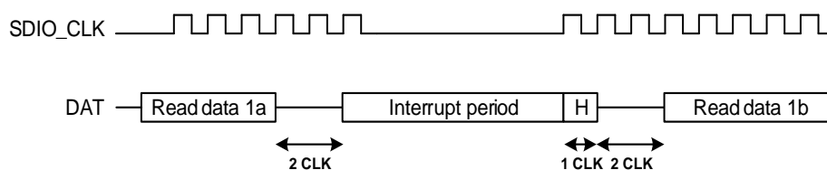
Figure 24-12. Read wait control by stopping SDIO_CLK
