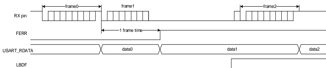
Figure 20-26. Break frame occurs during a frame
