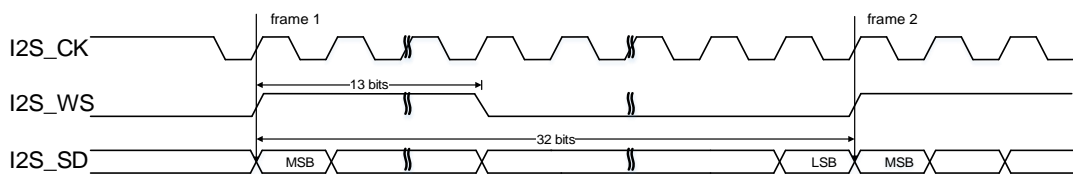
Figure 22-47. PCM standard long frame synchronization mode timing diagram
