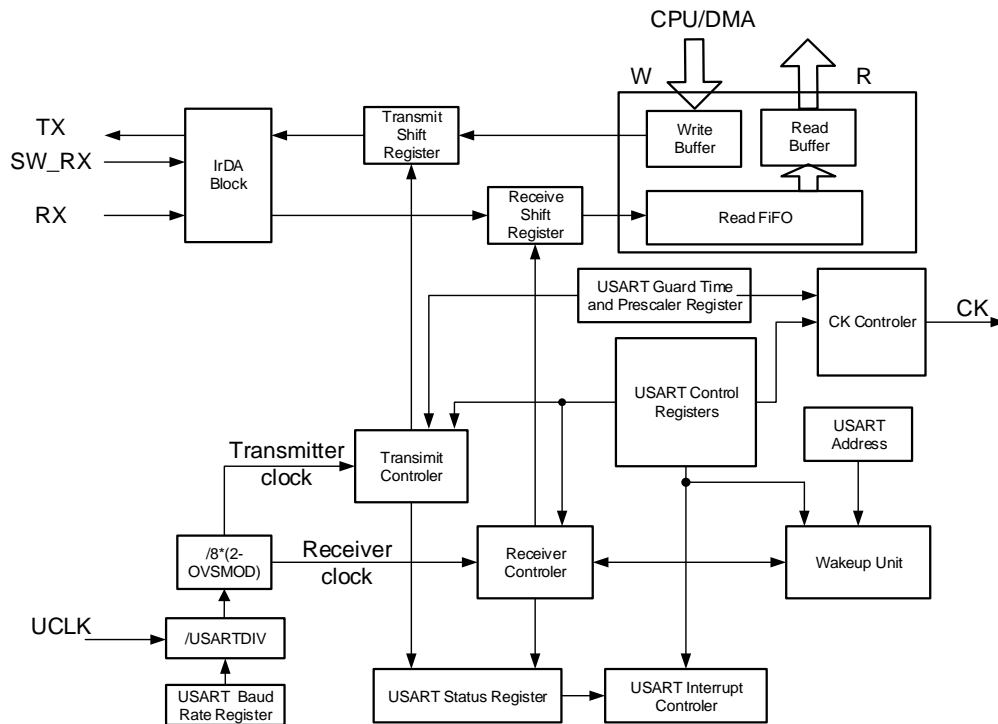
Figure 20-17. USART module block diagram
