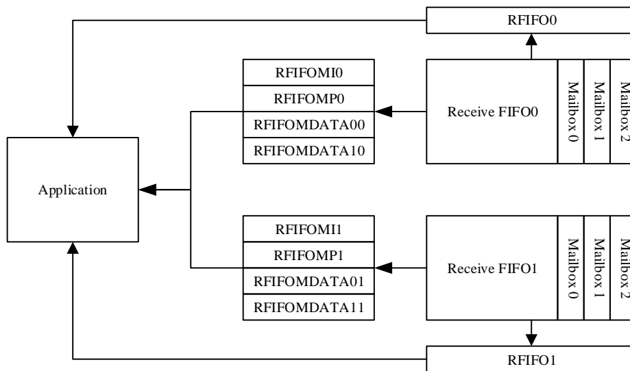
Figure 26-4. Reception register
