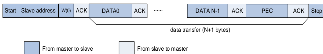
Figure 21-35. SMBus master transmitter and slave receiver communication flow
