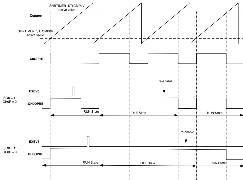
Figure 19-31. ISO0 = 1 and CHOP = 0 in delayed IDLE
