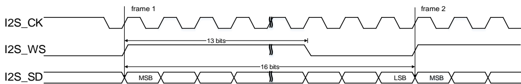
Figure 22-45. PCM standard long frame synchronization mode timing diagram (DTLEN=10, CHLEN=1, CKPL=0)
