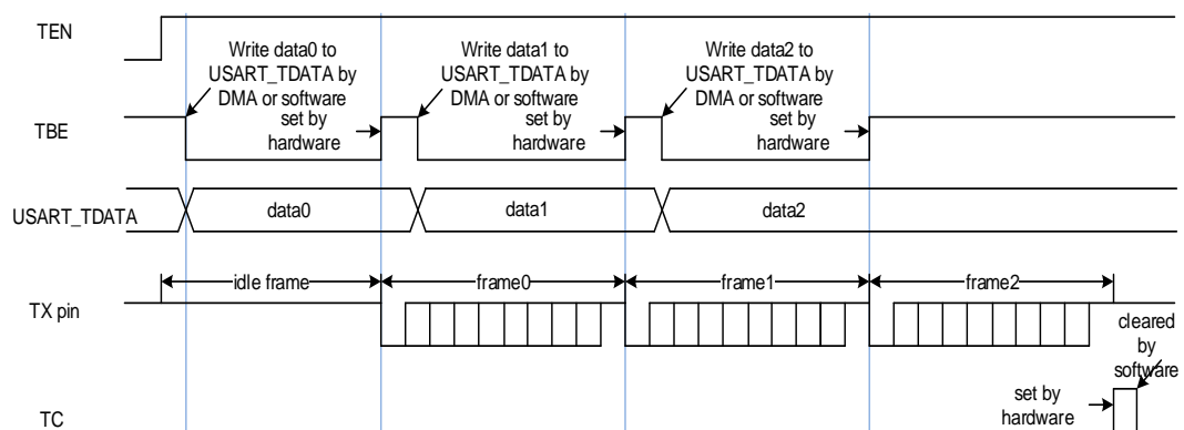
Figure 20-19. USART transmit procedure
