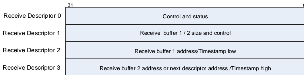
Figure 27-9. Receive descriptor in normal mode
