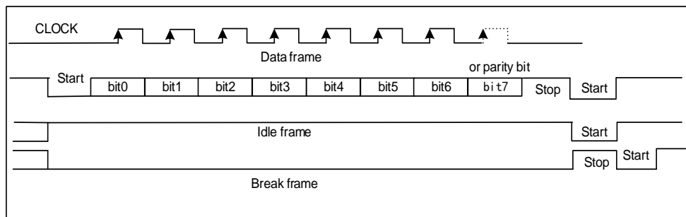
Figure 20-18. USART character frame (8 bits data and 1 stop bit)
