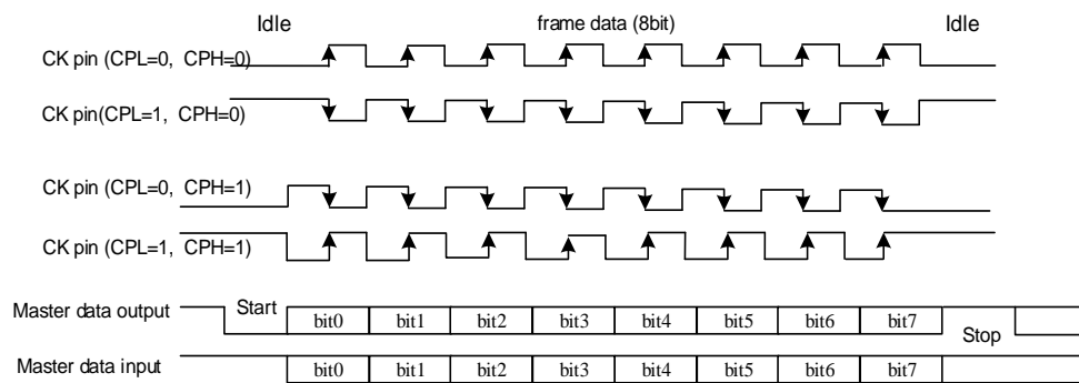
Figure 20-28. 8-bit format USART synchronous waveform (CLEN=1)
