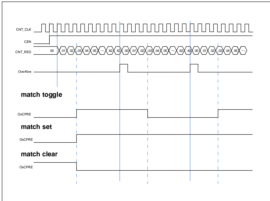
Figure 18-76. Output-compare in three modes
