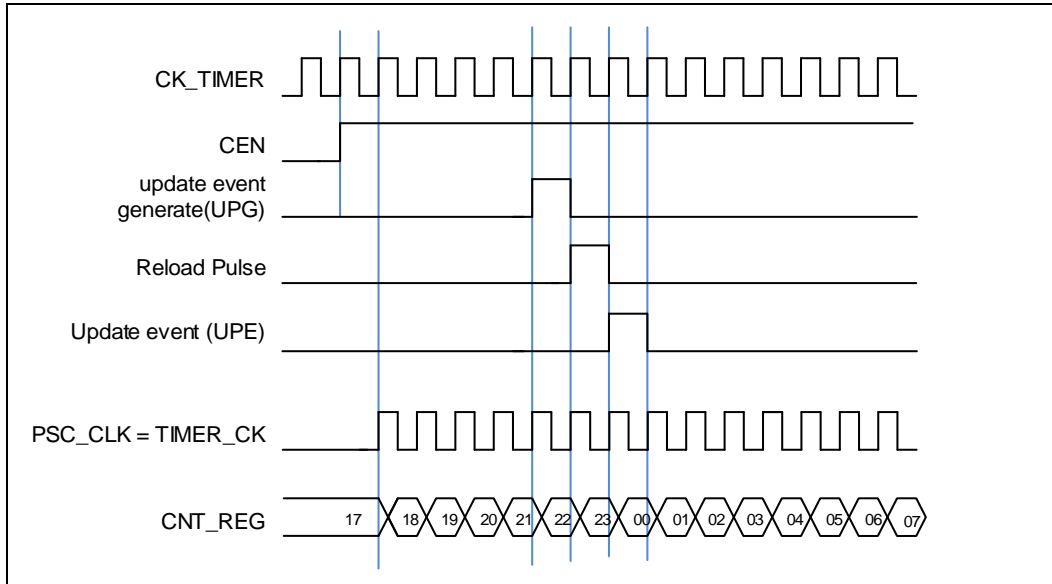
Figure 18-85. Timing chart of internal clock divided by 1
