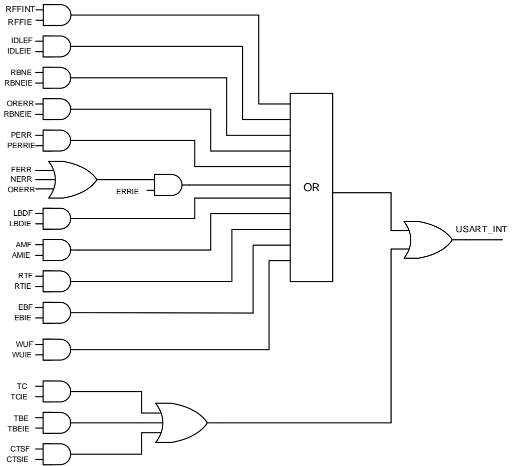
Figure 20-33. USART interrupt mapping diagram
