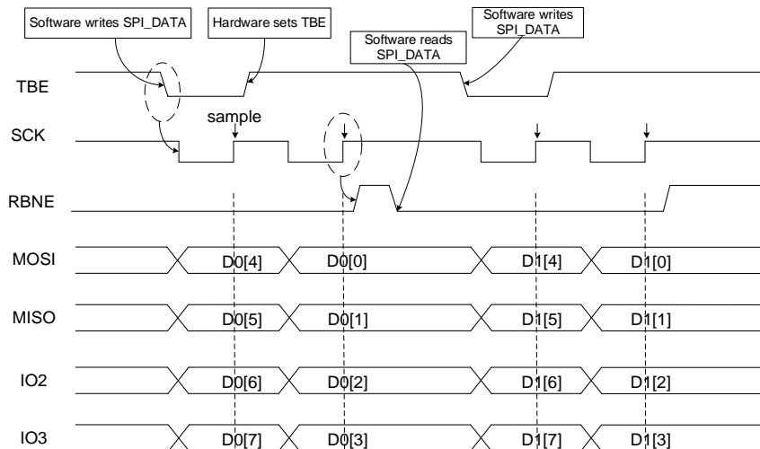
Figure 22-13. Timing diagram of read operation in Quad-SPI mode
