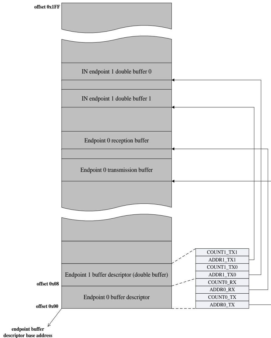
Figure 28-2. An example with buffer descriptor table usage (USB_BADDR = 0)
