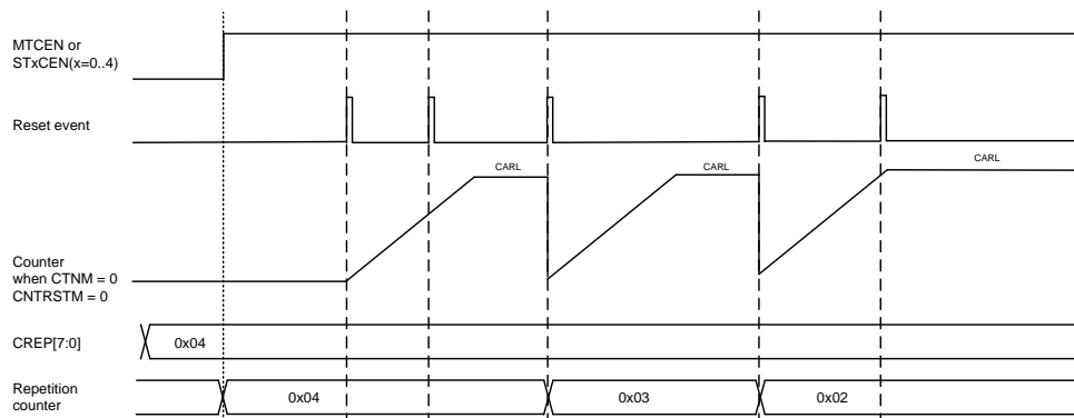
Figure 19-7. Repetition counter behavior in single pulse mode with CNTRSTM = 0
