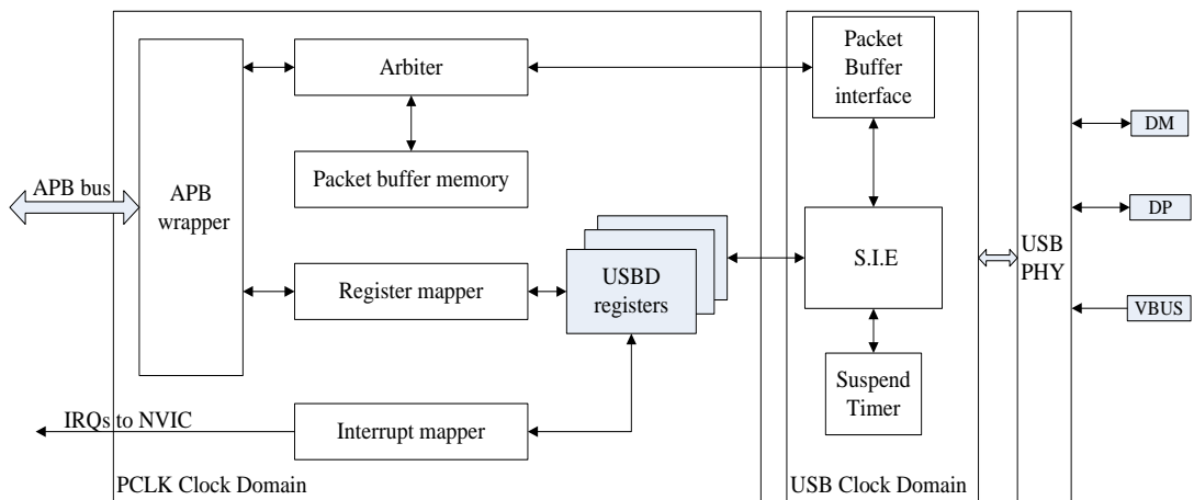
Figure 28-1. USB D block diagram
