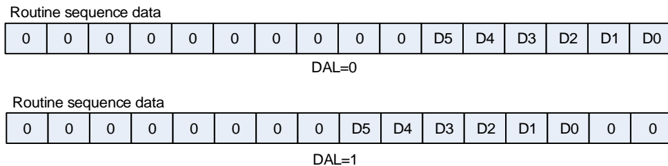
Figure 13-9. 6-bit data storage mode
