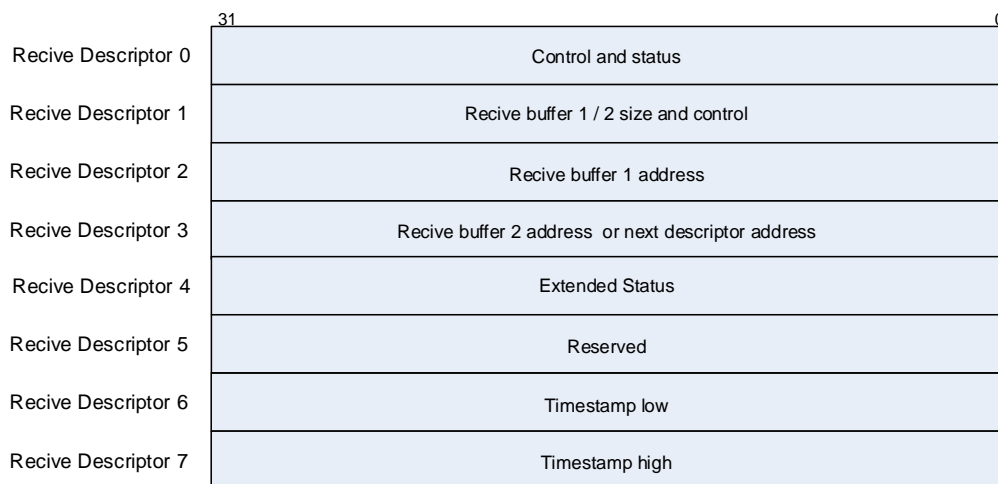
Figure 27-10. Receive descriptor in enhanced mode
