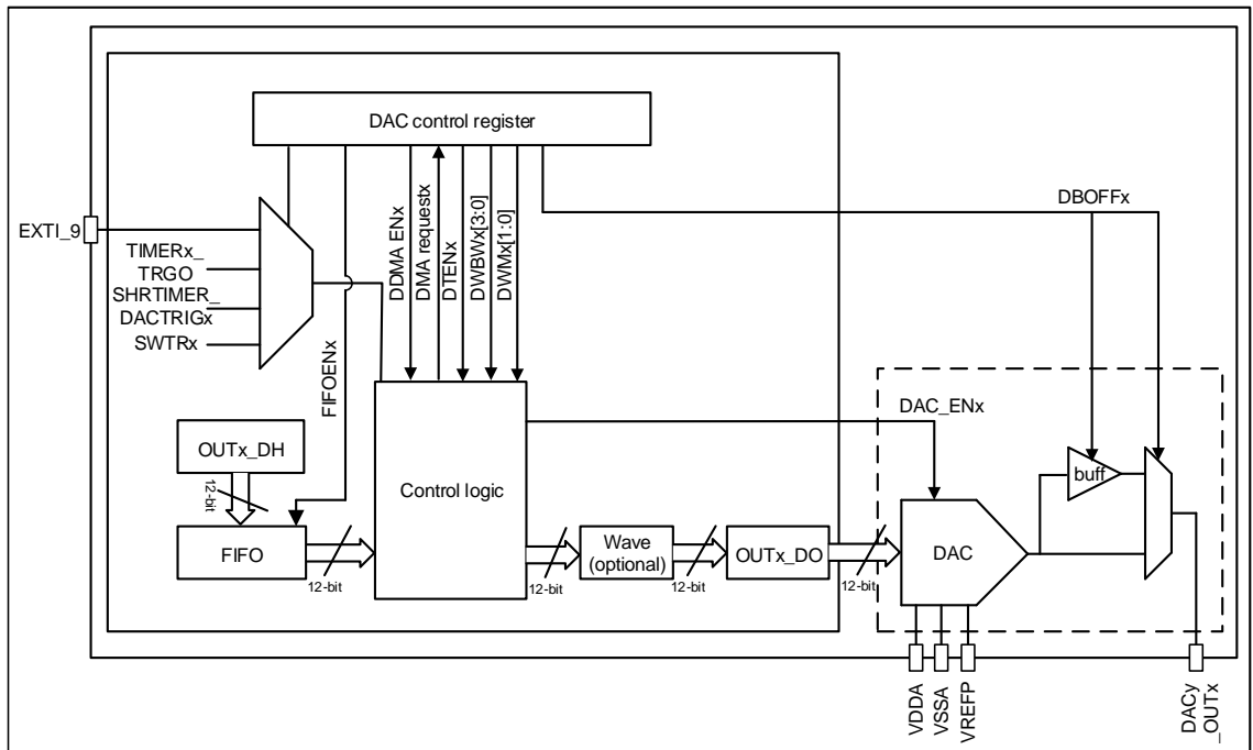
Figure 14-1. DAC block diagram
