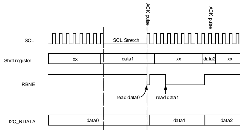
Figure 21-25. Data reception
