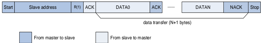
Figure 21-19. I2C communication flow with 7-bit address (Master Receive)
