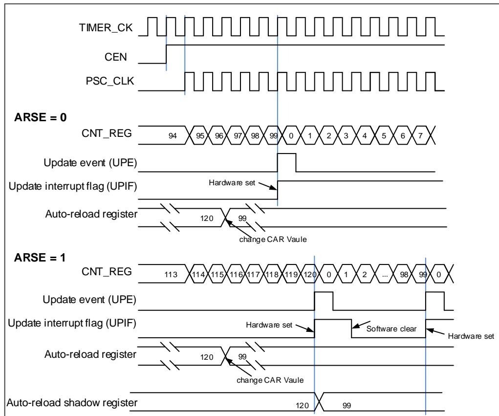
Figure 18-101. Timing chart of up counting mode, change TIMERx_CAR ongoing
