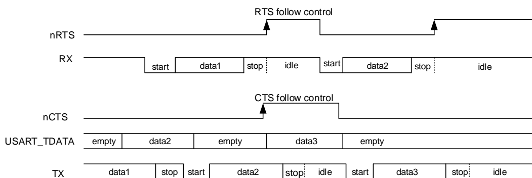
Figure 20-24. Hardware flow control
