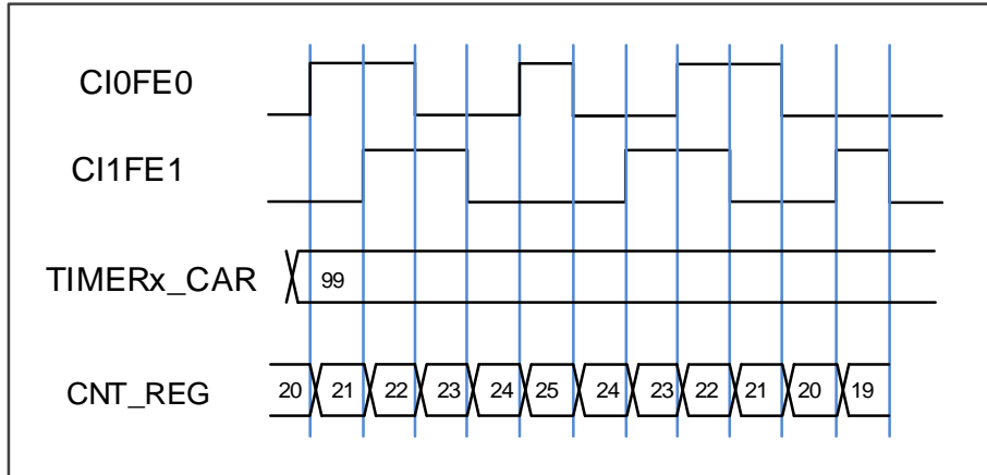
Figure 18-20. Counter behavior with CI0FE0 polarity non-inverted in mode 2
