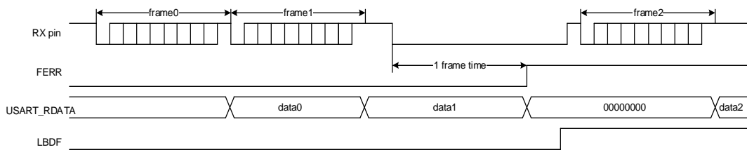
Figure 20-25. Break frame occurs during idle state
