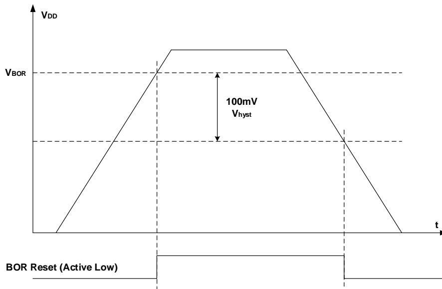
Figure 4-2. Waveform of the BOR
