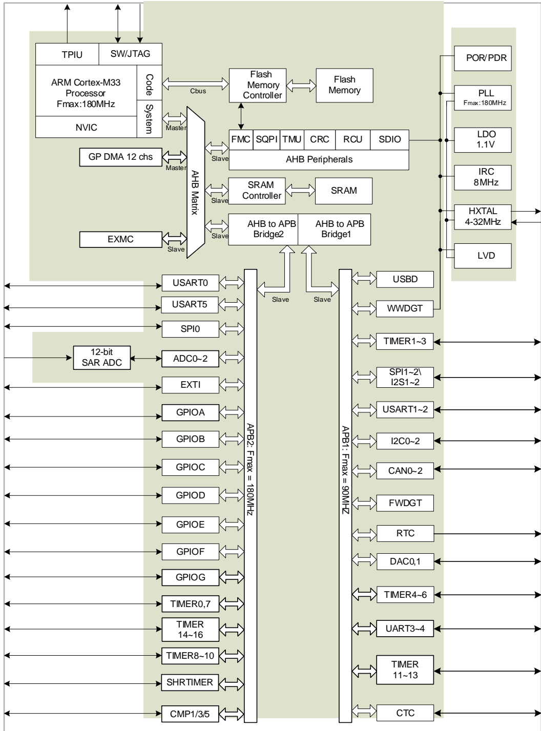
Figure 1-2. High density devices system architecture
