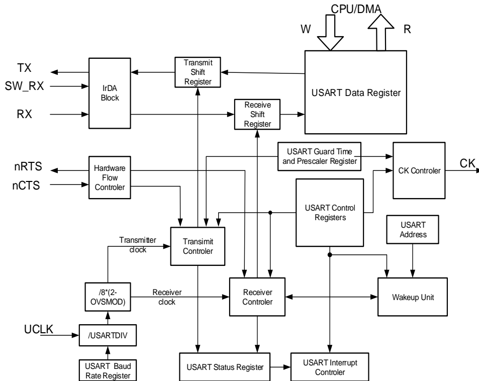
Figure 20-1. USART module block diagram
