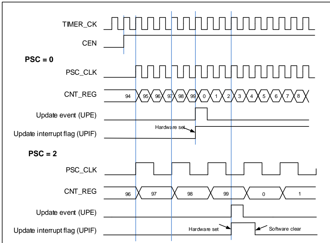
Figure 18-87. Timing chart of up counting mode, PSC=0/2
