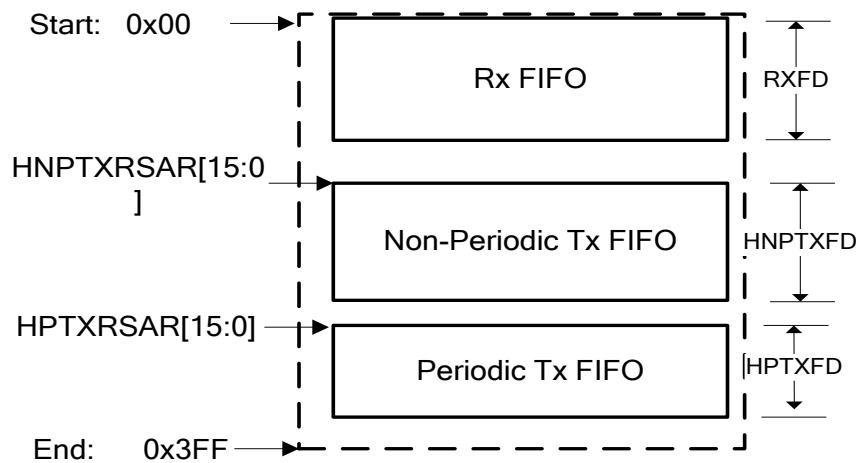
Figure 29-6. Host mode FIFO space in SRAM
