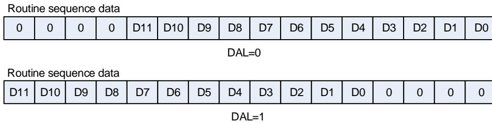
Figure 13-8. 12-bit data storage mode
