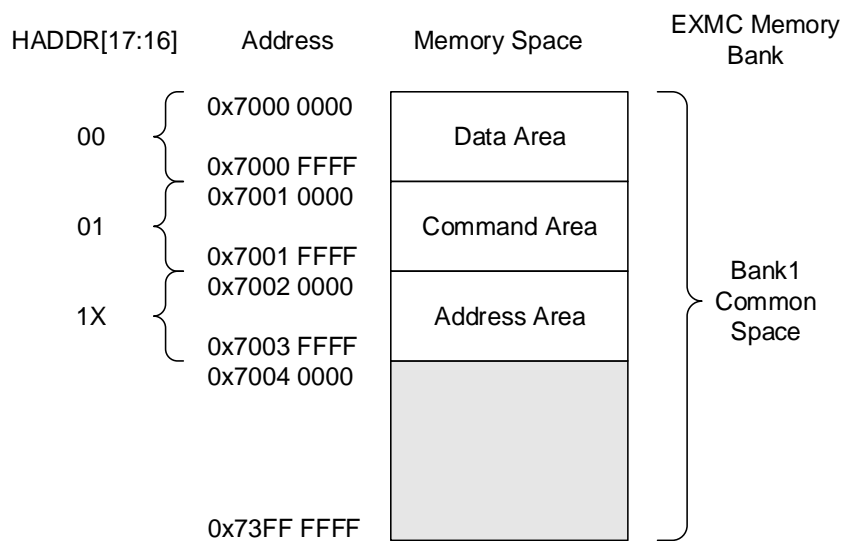
Figure 25-5. Diagram of bank1 common space
