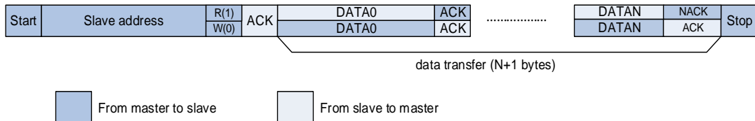
Figure 21-7. I2C communication flow with 10-bit address (Master Transmit)
