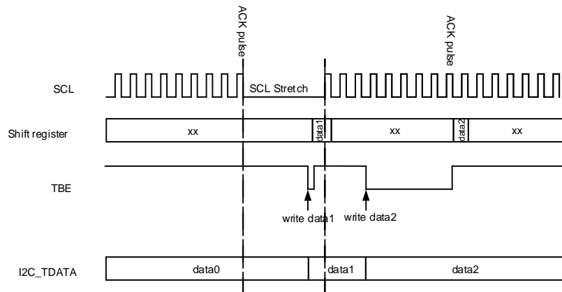
Figure 21-24. Data transmission
