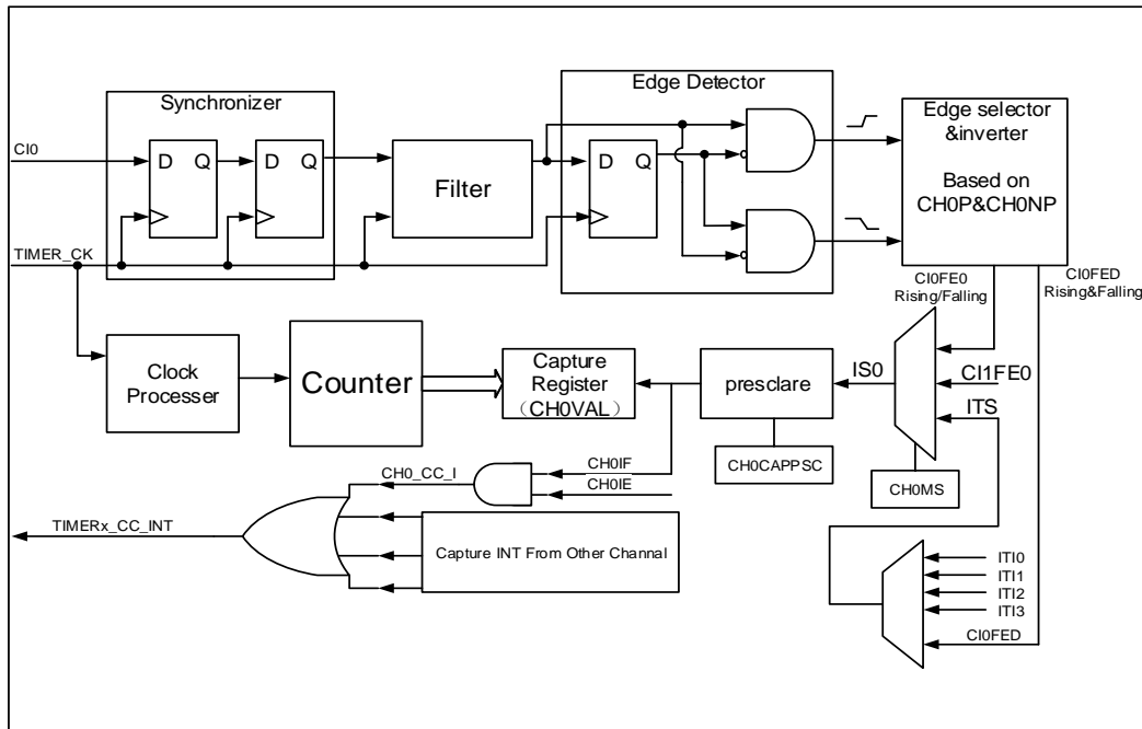
Figure 18-73. Channel input capture principle
