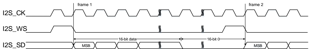
Figure 22-42. PCM standard short frame synchronization mode timing diagram
