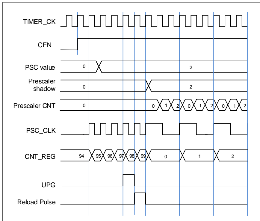
Figure 18-86. Timing chart of PSC value change from 0 to 2
