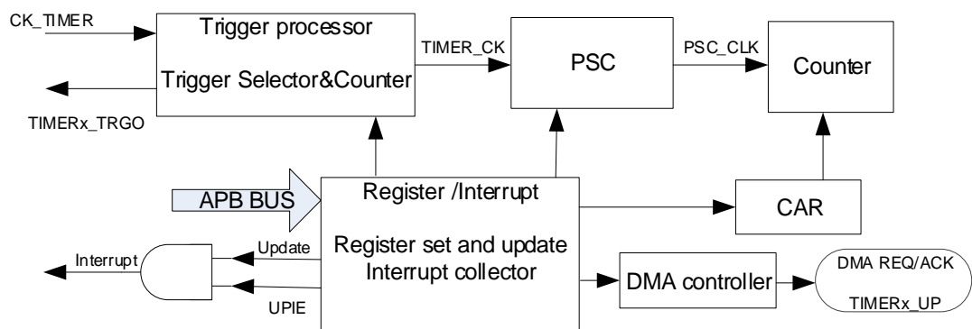
Figure 18-97. Basic timer block diagram
