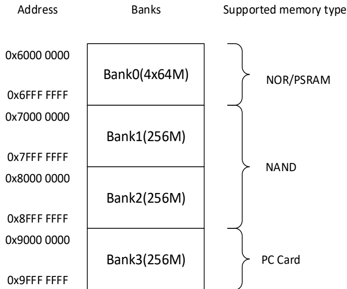
Figure 25-2. EXMC memory banks
