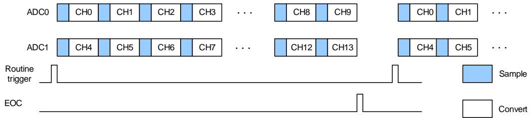
Figure 13-13. Routine parallel mode on 10 channels
