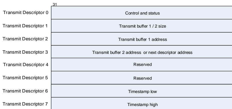
Figure 27-8. Transmit descriptor in enhanced mode
