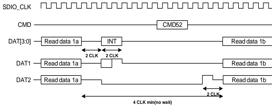
Figure 24-13. Read wait operation using SDIO_DAT[2]
