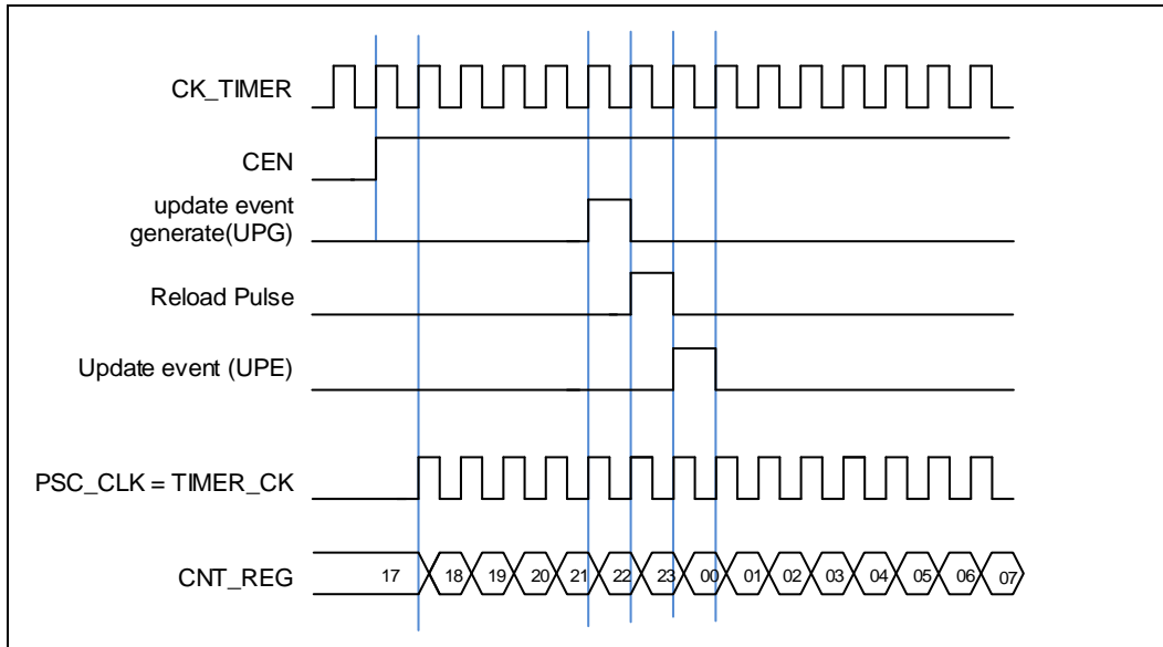
Figure 18-98. Timing chart of internal clock divided by 1
