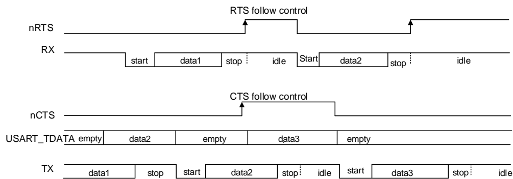
Figure 20-8. Hardware flow control
