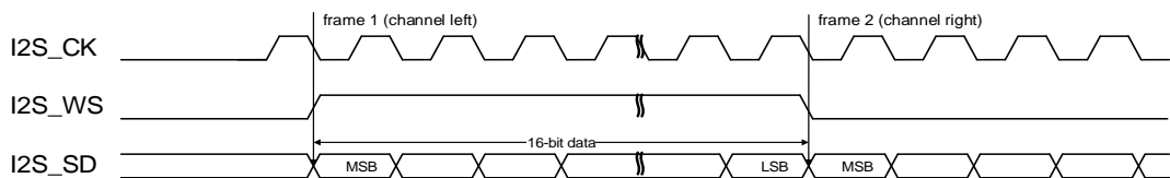
Figure 22-23. MSB justified standard timing diagram (DTLEN=00, CHLEN=0, CKPL=0)
