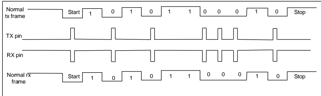
Figure 20-14. IrDA data modulation
