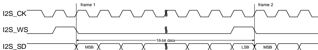
Figure 22-37. PCM standard short frame synchronization mode timing diagram
