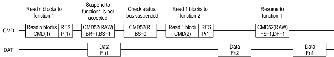
Figure 24-14. Function2 read cycle inserted during function1 multiple read cycle
