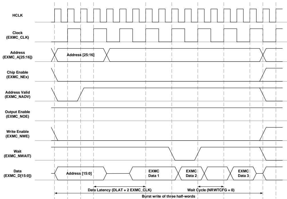
Figure 25-22. Write timing of synchronous multiplexed burst mode
