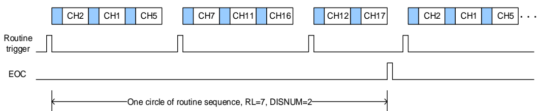
Figure 13-7. Discontinuous operation mode
