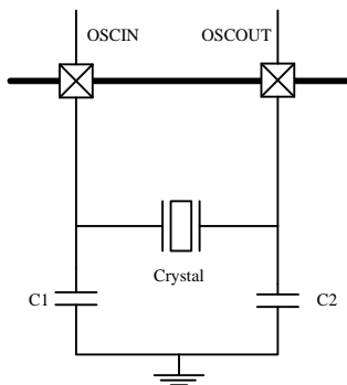
Figure 5-7. HXTAL clock source
