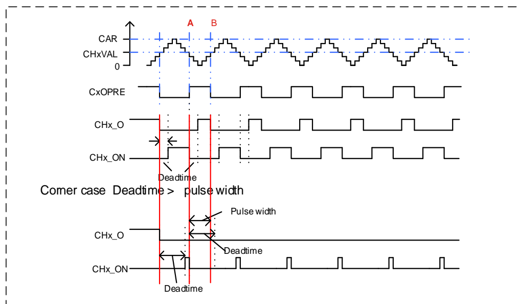
Figure 18-78. Complementary output with dead-time insertion
