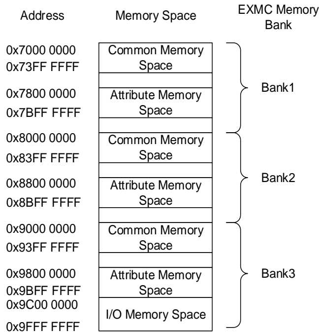
Figure 25-4. NAND/PC Card address mapping
