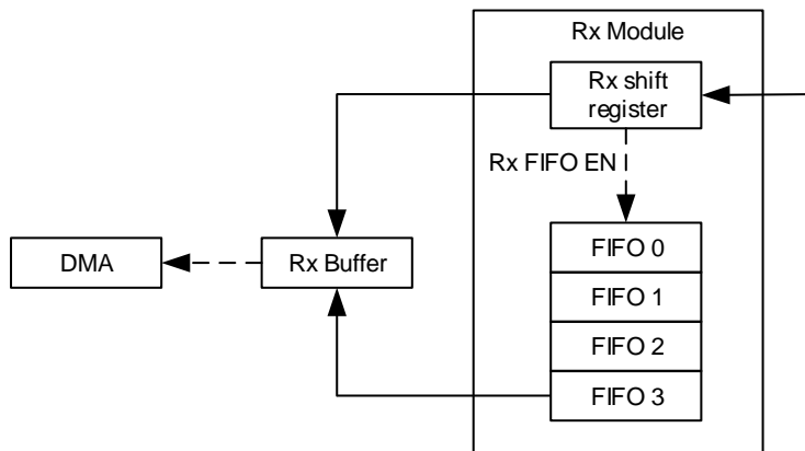
Figure 20-32. USART Receive FIFO structure
