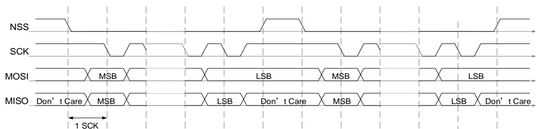
Figure 22-11. Timing diagram of NSS pulse with continuous transmit
