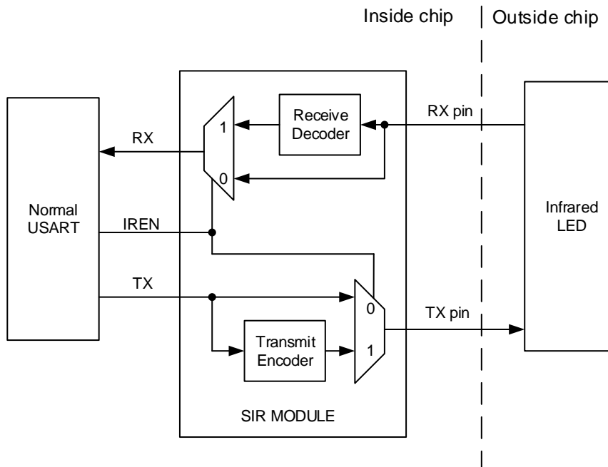
Figure 20-29. IrDA SIR ENDEC module
