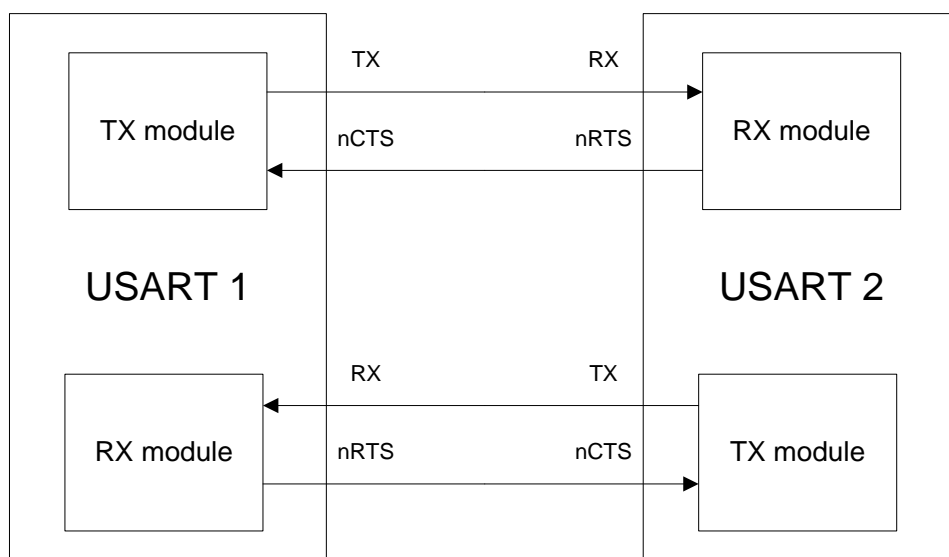
Figure 20-23. Hardware flow control between two USARTs
