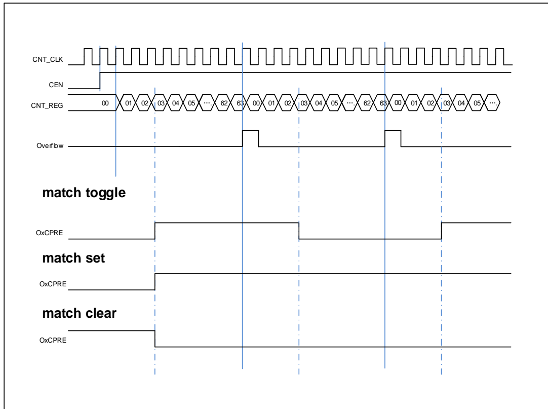
Figure 18-92. Output-compare under three modes
