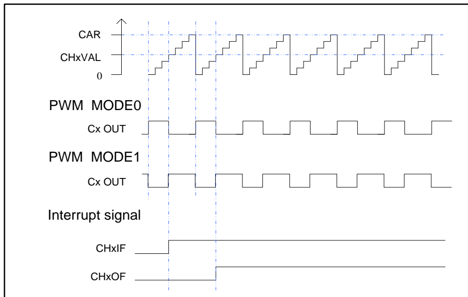
Figure 18-93. PWM mode timechart
