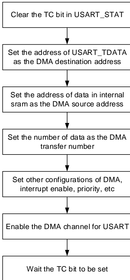
Figure 20-21. Configuration step when using DMA for USART transmission
