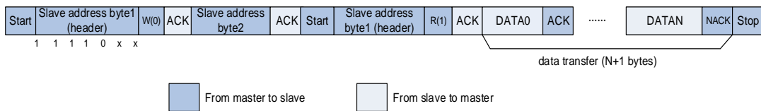
Figure 21-8. I2C communication flow with 10-bit address (Master Receive)
