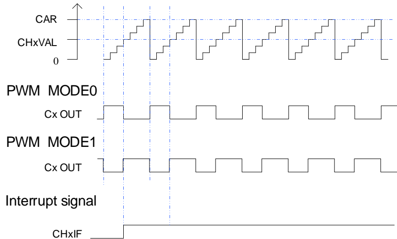
Figure 18-54. PWM mode timechart
