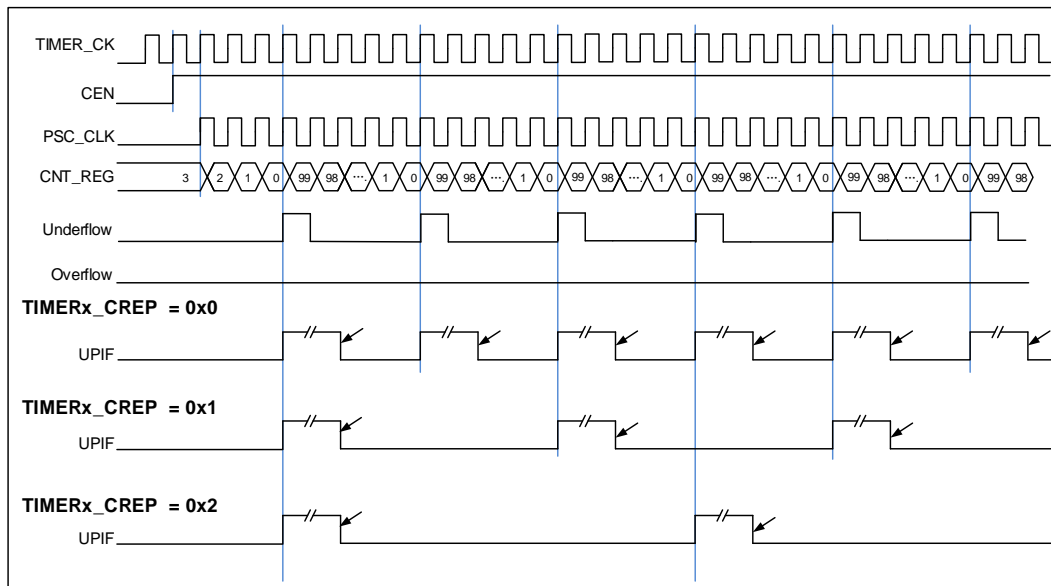
Figure 18-11. Repetition timechart for down-counter
