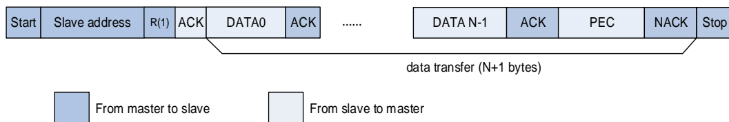
Figure 21-36. SMBus master receiver and slave transmitter communication flow
