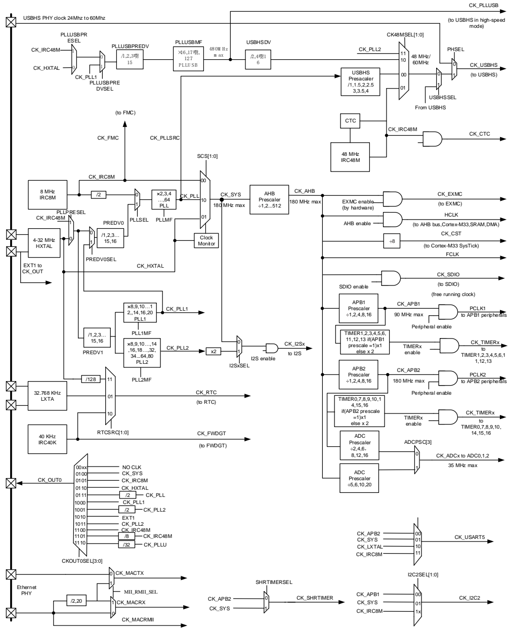
Figure 5-6. Clock tree
