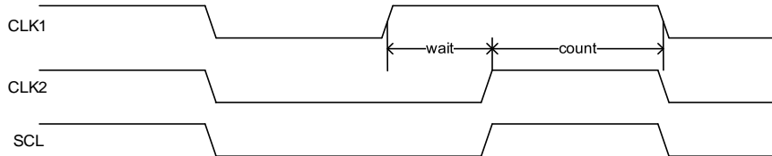
Figure 21-4. Clock synchronization
