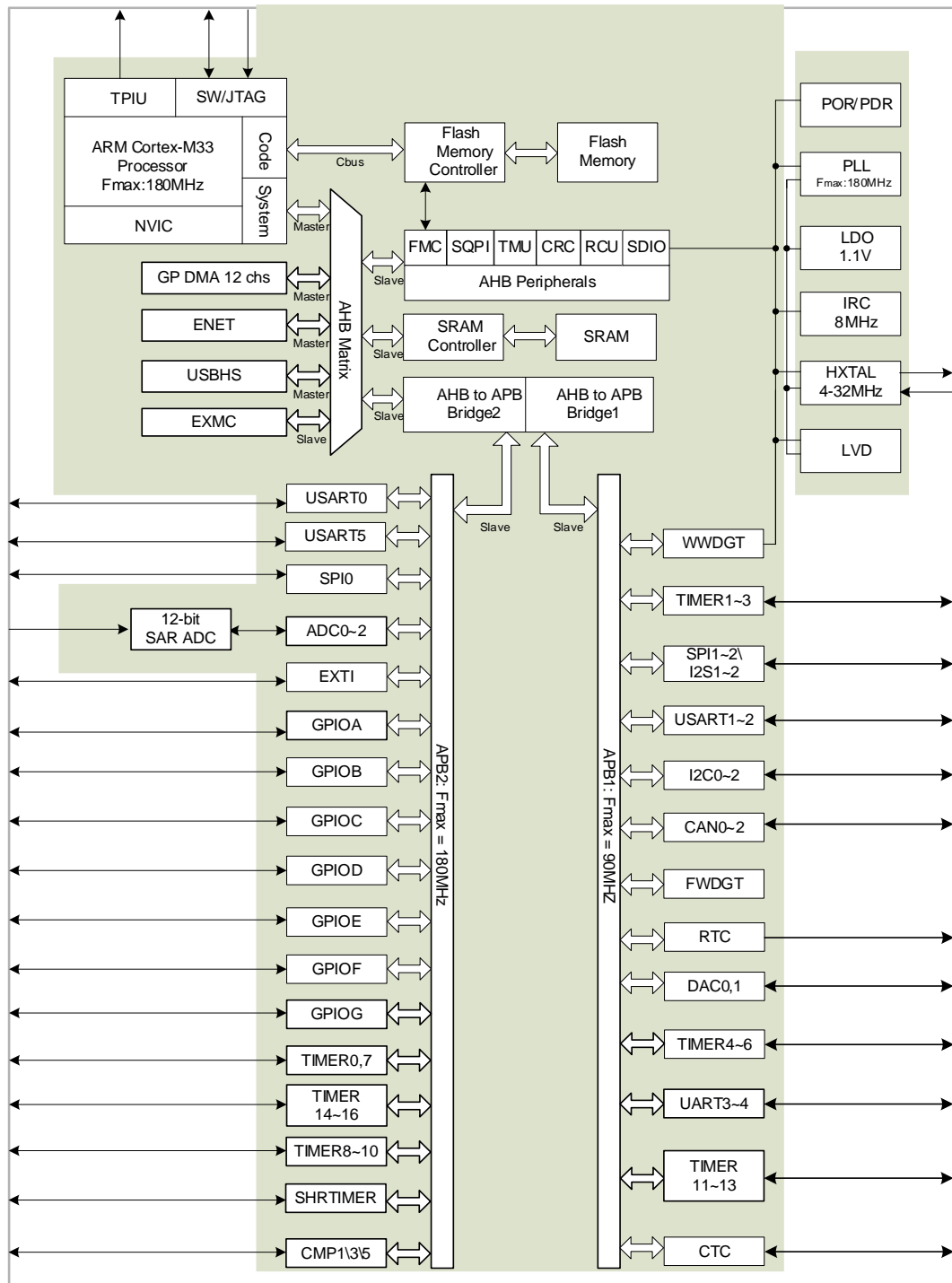
Figure 1-3. Connectivity line devices system architecture
