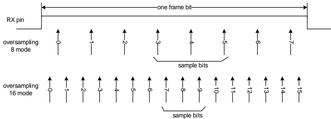
Figure 20-20. Oversampling method of a receive frame bit (OSB=0)
