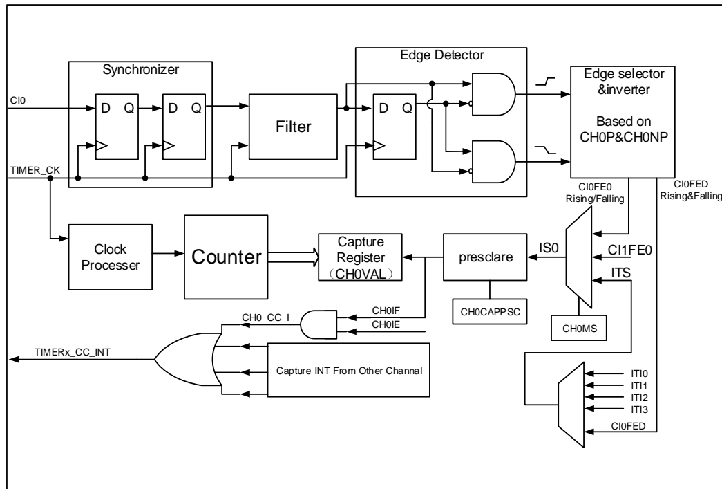
Figure 18-90. Channel input capture principle
