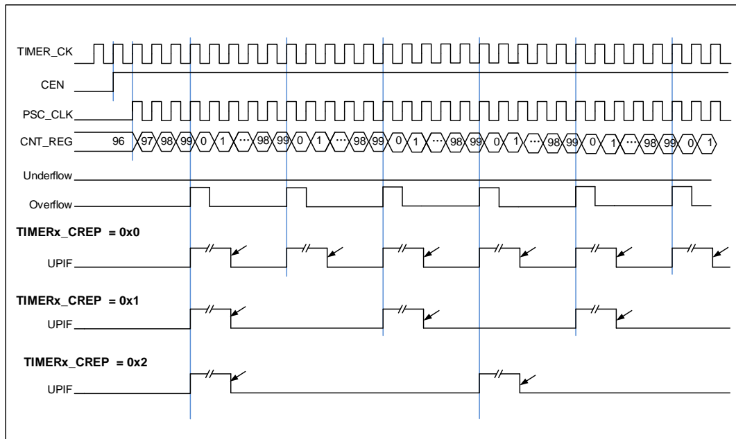
Figure 18-72. Repetition counter timing chart of up counting mode
