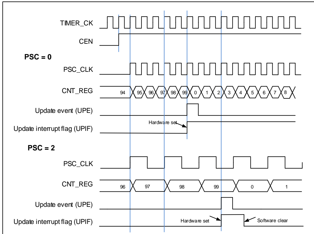
Figure 18-33. Timing chart of up counting mode, PSC=0/2
