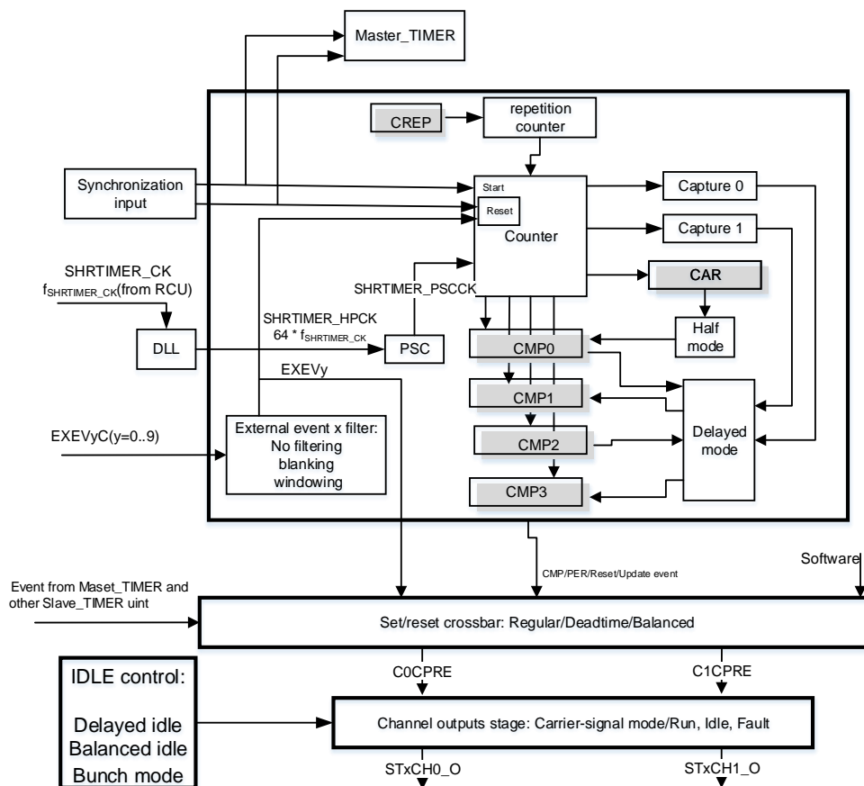
Figure 19-10. Slave_TIMER x diagram
