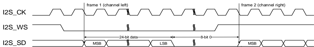
Figure 22-20. I2S Phillips standard timing diagram (DTLEN=01, CHLEN=1, CKPL=1)
