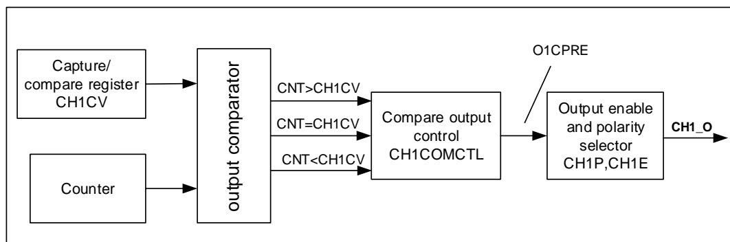
Figure 18-75. Channel output compare principle (CH1_O)
