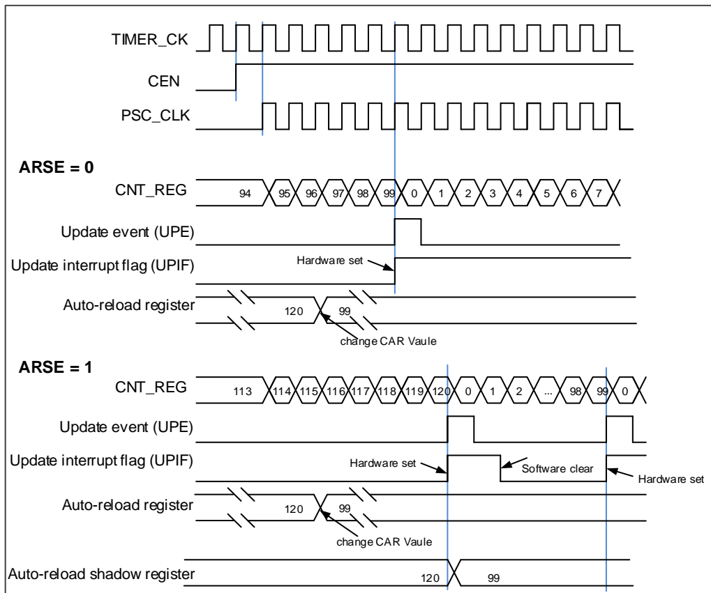
Figure 18-88. Timing chart of up counting mode, change TIMERx_CAR ongoing
