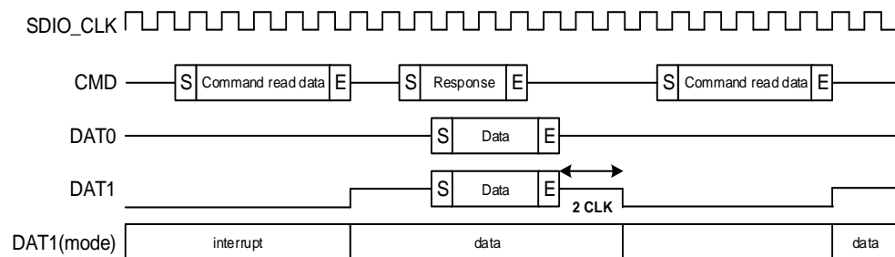
Figure 24-15. Read Interrupt cycle timing
