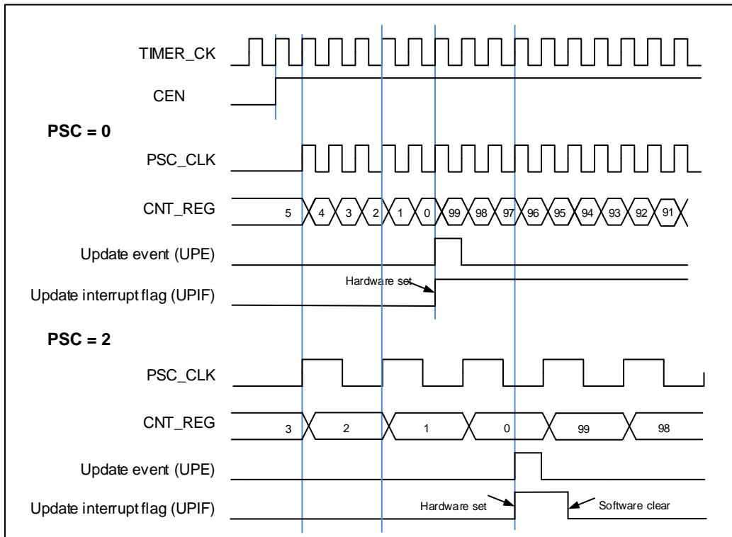
Figure 18-35. Timing chart of down counting mode,PSC=0/2
