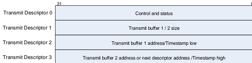
Figure 27-7. Transmit descriptor in normal mode
