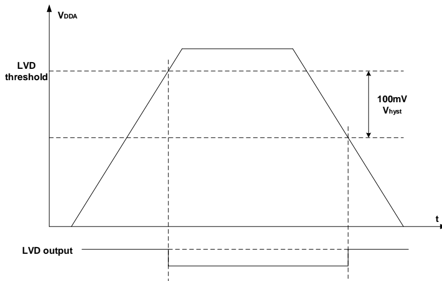
Figure 4-4. Waveform of the LVD threshold
