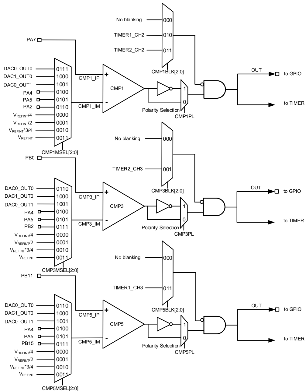
Figure 15-1. CMP block diagram
