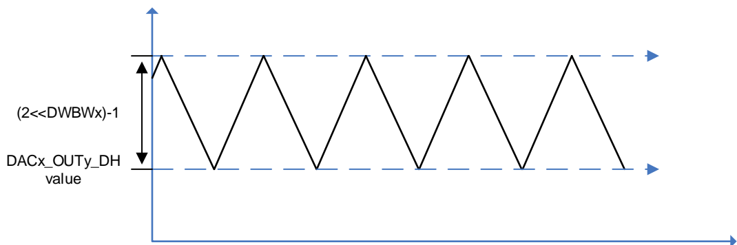
Figure 14-3. DAC triangle noise wave
