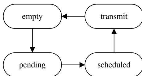
Figure 26-3. State of transmit mailbox
