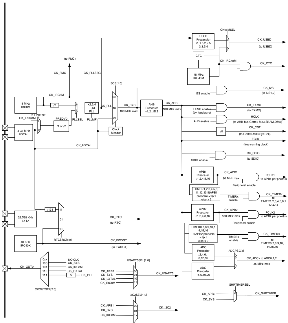
Figure 5-2. Clock tree
