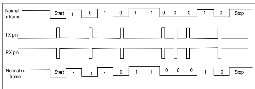
Figure 20-30. IrDA data modulation
