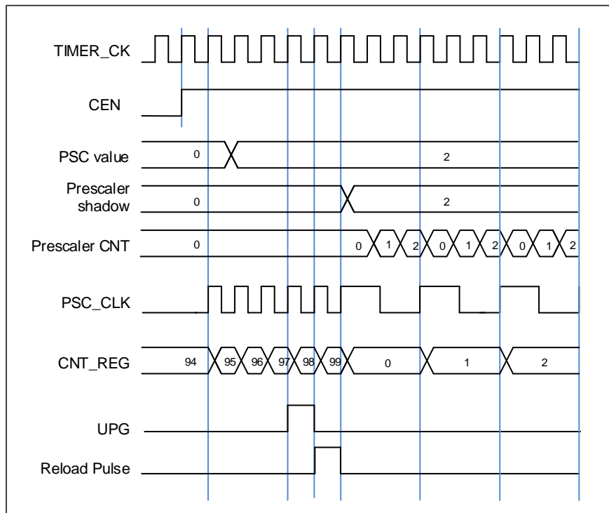
Figure 18-99. Timing chart of PSC value change from 0 to 2
