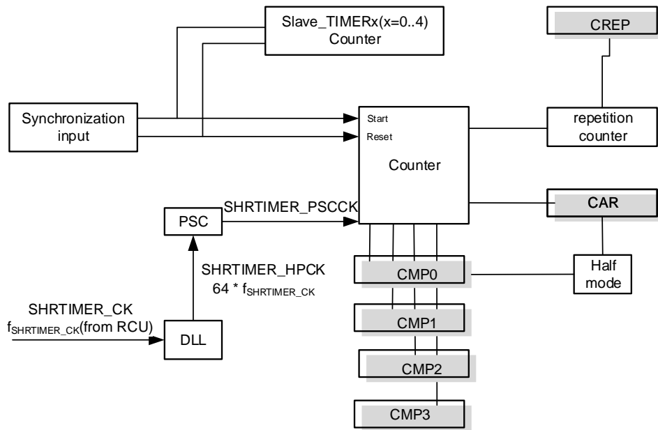
Figure 19-2. Master_TIMER diagram
