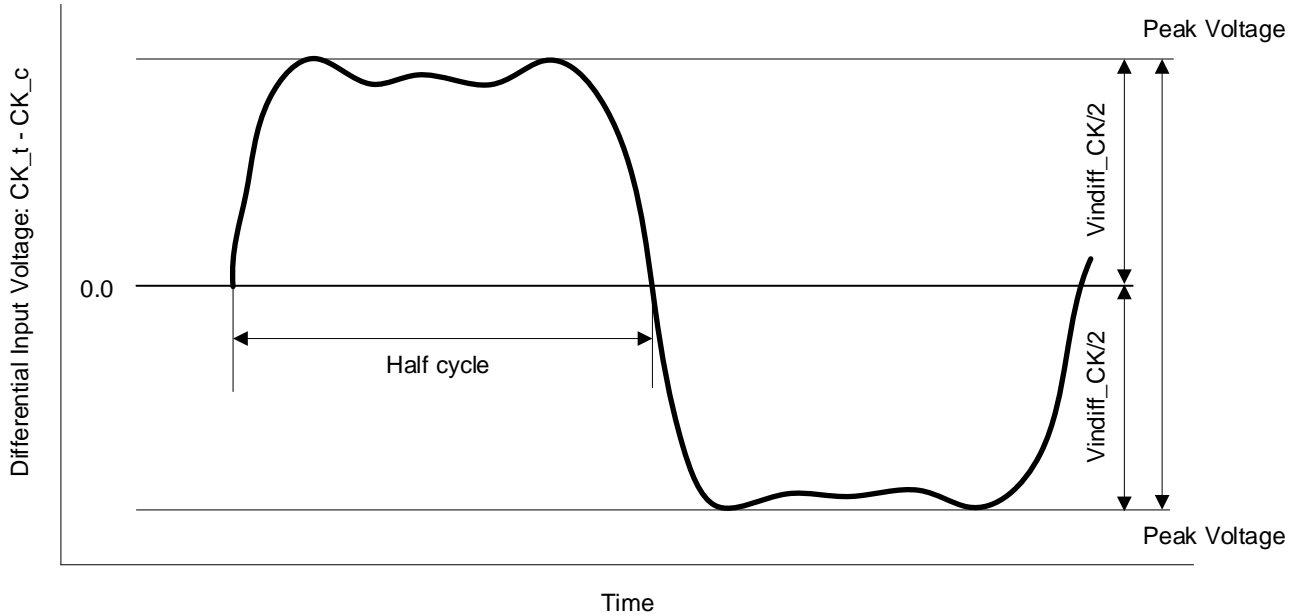
Figure 5-4 CK Differential Input Voltage
