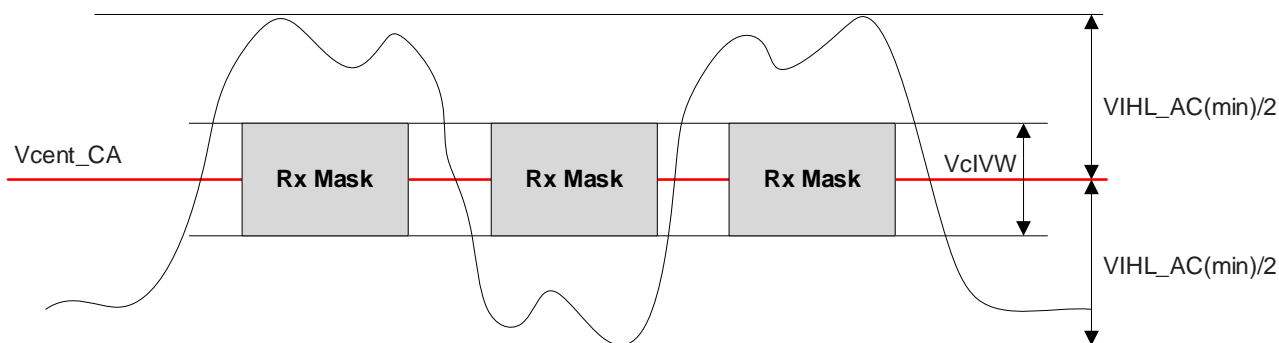
Figure 8-5 CA VIH_L_AC Definition (for Each Input Pulse)
