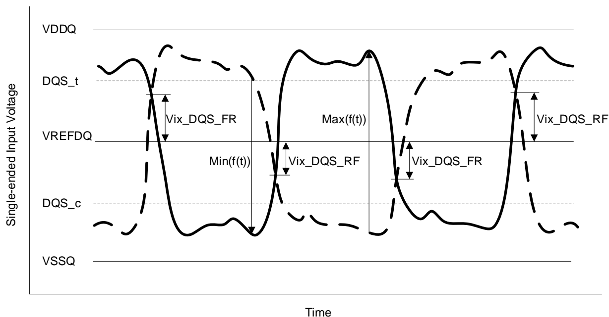
Figure 5-13 Vix Definition (DQS)
