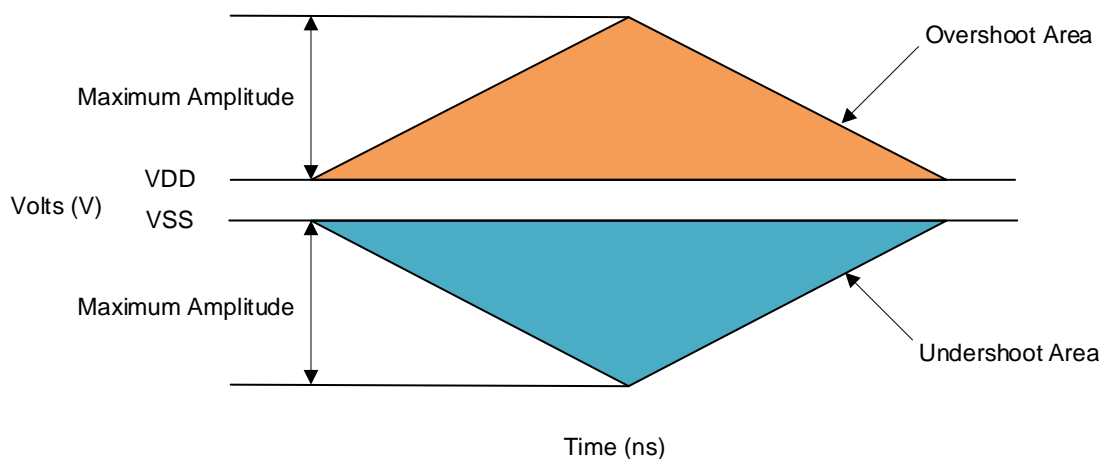
Figure 5-3 AC Overshoot and Undershoot Definition for Address and Control Pins
