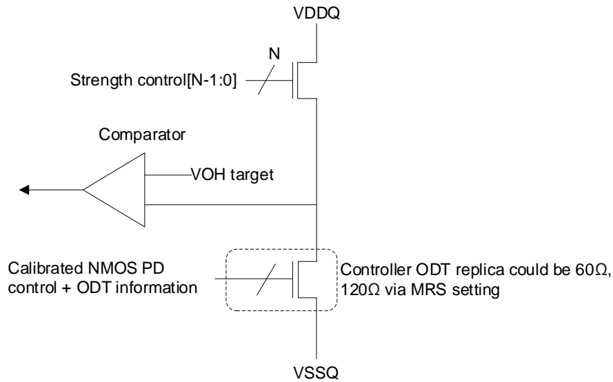
Figure 5-20 Pull-up Calibration
