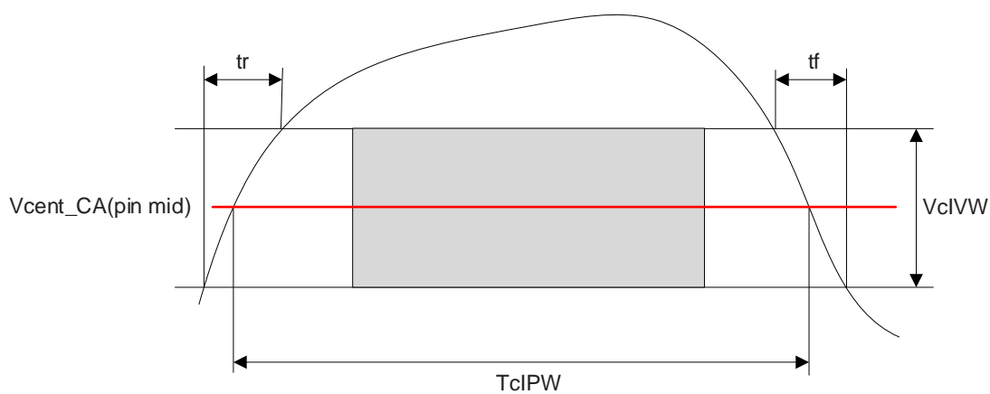
Figure 8-4 CA TcIPW and SRIN_cIVW definition (for each input pulse)
