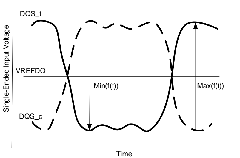
Figure 5-10 Definition of Differential DQS Peak Voltage
