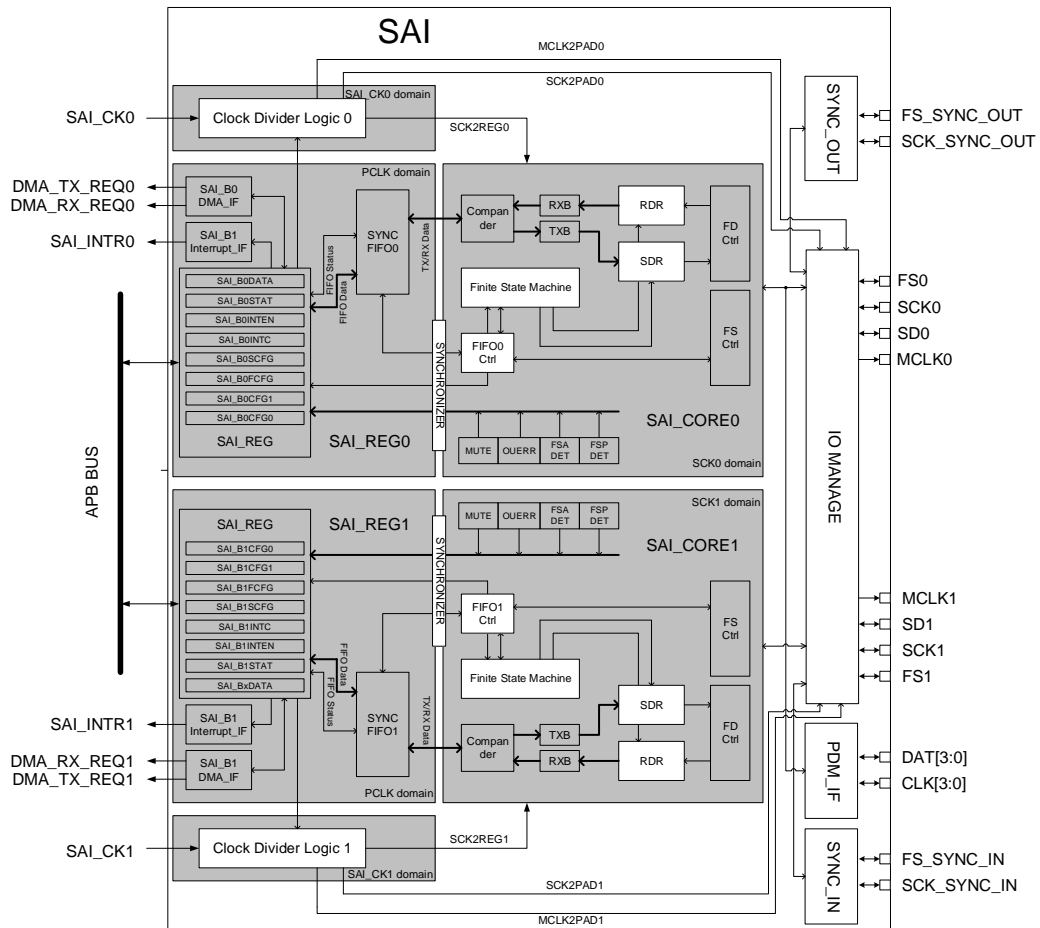
Figure 26-1. block diagram
