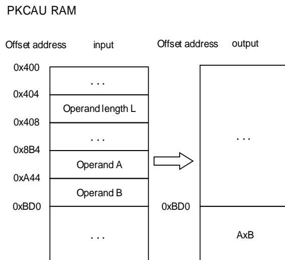
Figure 11-7. Arithmetic multiplication
