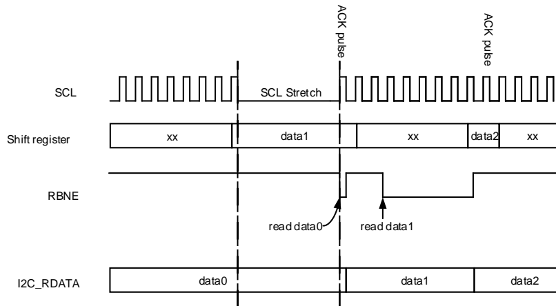
Figure 24-25. Data reception
