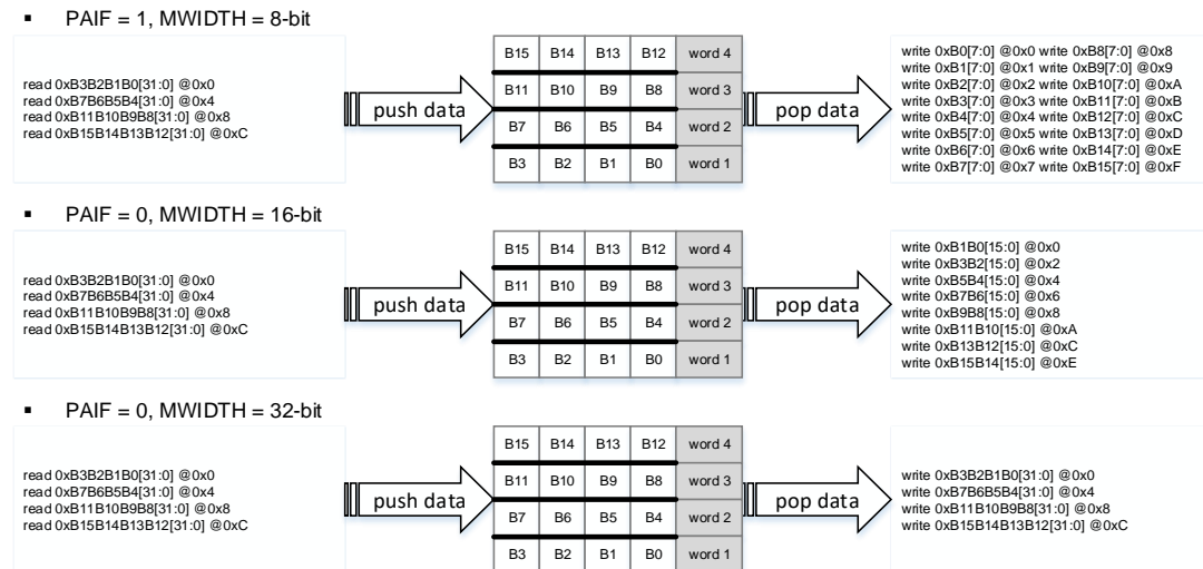
Figure 14-6. Data packing/unpacking when PWIDTH = '10'
