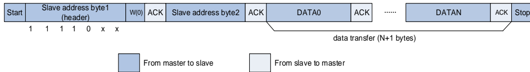
Figure 24-7. I2C communication flow with 10-bit address (Master Transmit)
