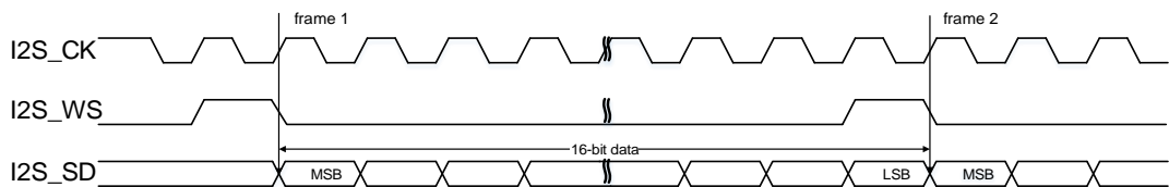
Figure 25-35. PCM standard short frame synchronization mode timing diagram (DTLEN=00, CHLEN=0, CKPL=1)
