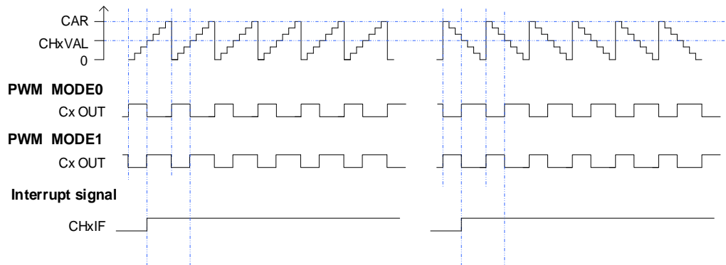
Figure 22-15. CAPWM timechart
