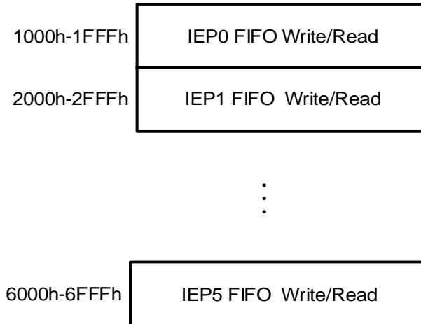
Figure 34-9. Device mode FIFO access register map
