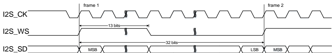
Figure 25-45. PCM standard long frame synchronization mode timing diagram (DTLEN=10, CHLEN=1, CKPL=1)
