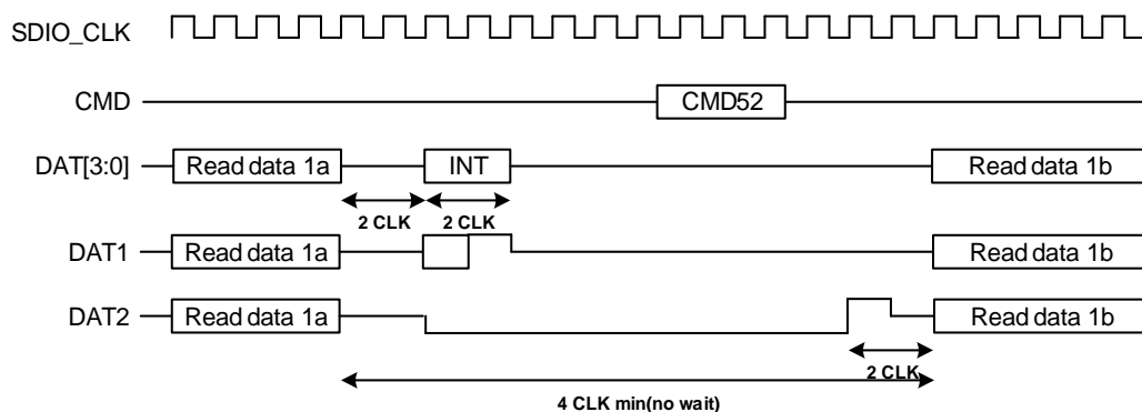
Figure 29-13. Read wait operation using SDIO_DAT[2]
