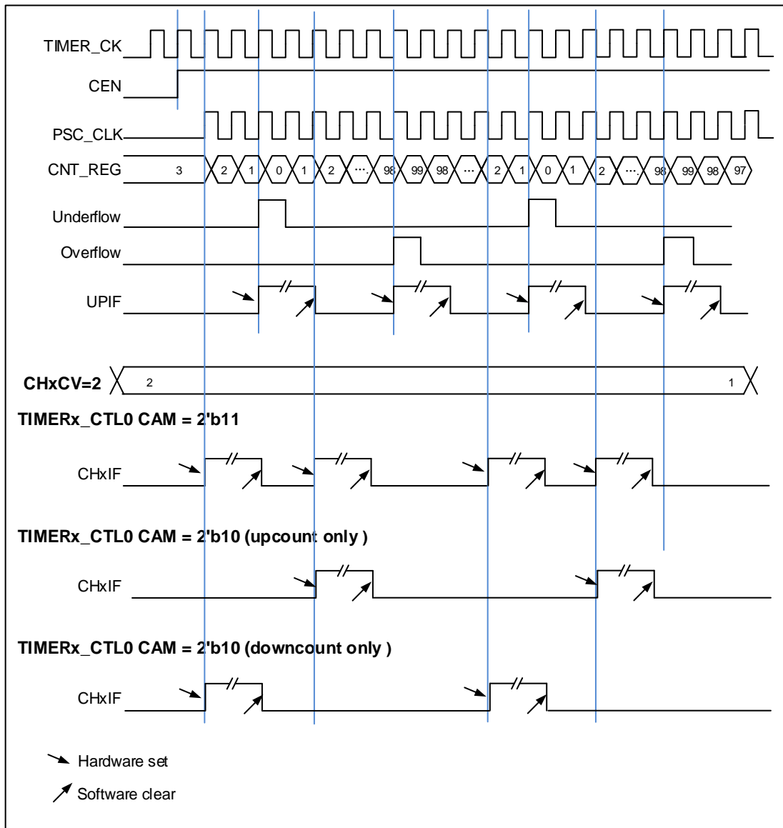
Figure 22-8. Center-aligned counter timechart
