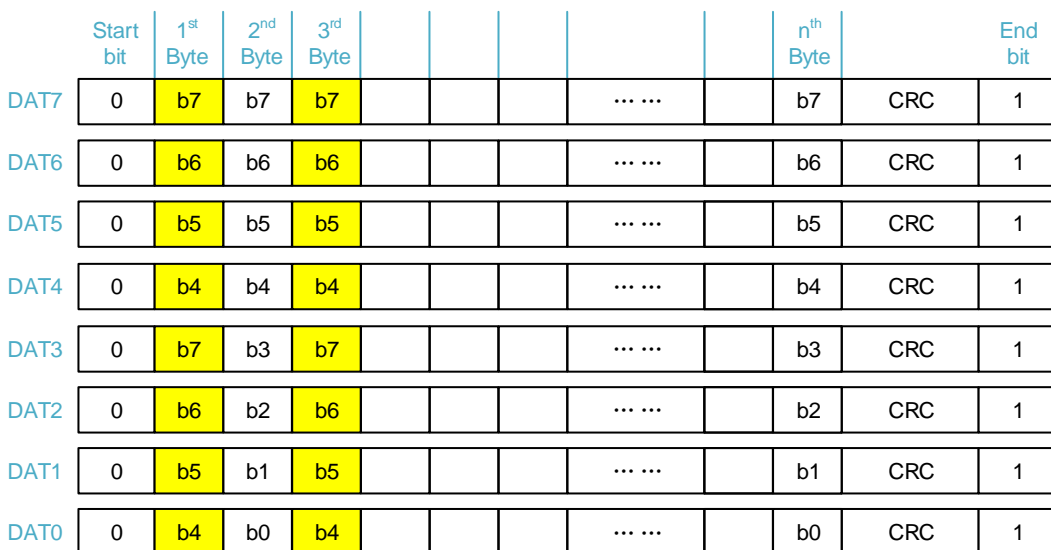
Figure 29-11. 8-bit data bus width
