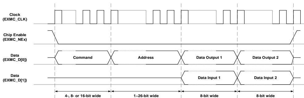
Figure 30-24. SPI-PSRAM access
