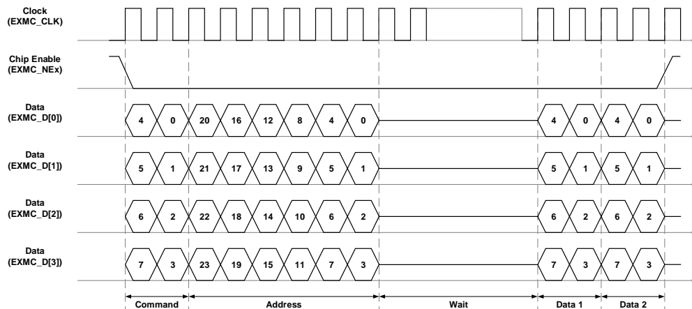
Figure 30-26. QPI-PSRAM access
