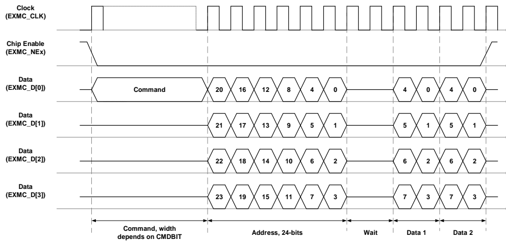
Figure 30-25. SQPI-PSRAM access
