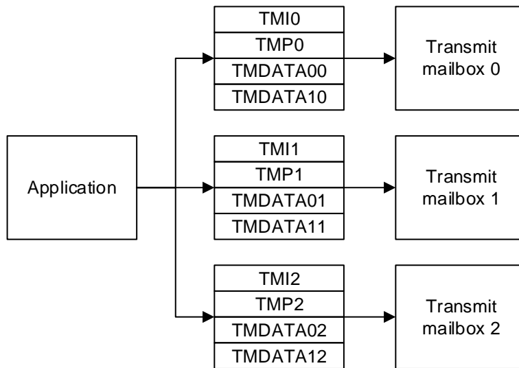
Figure 31-2. Transmission register
