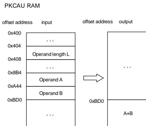
Figure 11-5. Arithmetic addition
