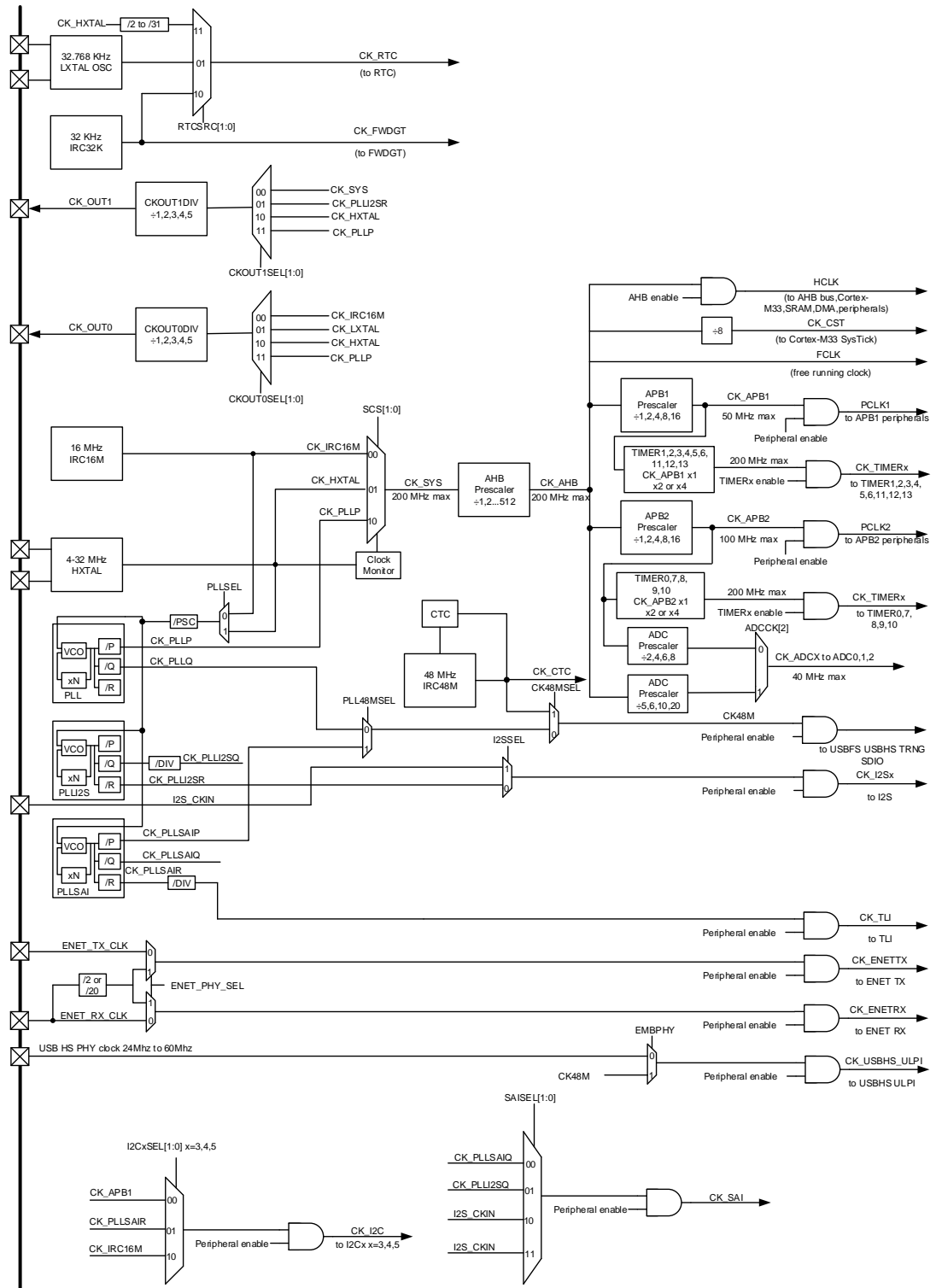
Figure 5-2. Clock tree
