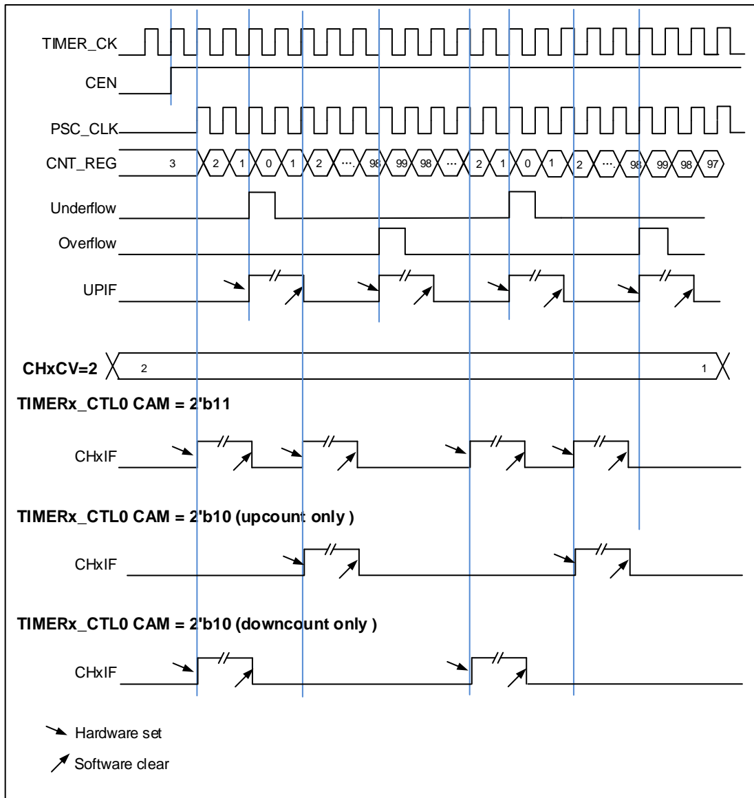
Figure 22-41. Timing chart of center-aligned counting mode
