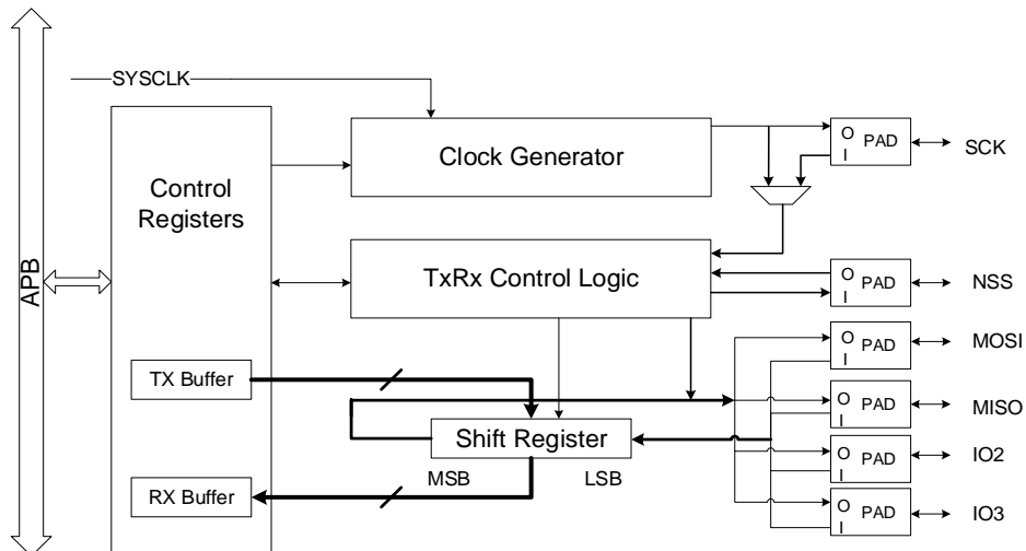
Figure 25-1. Block diagram of SPI
