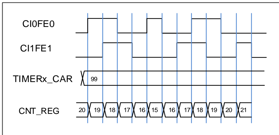
Figure 22-25. Counter behavior with CI0FE0 polarity inverted in mode 2
