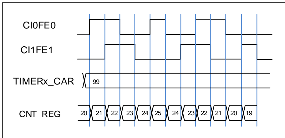
Figure 22-24. Counter behavior with CI0FE0 polarity non-inverted in mode 2
