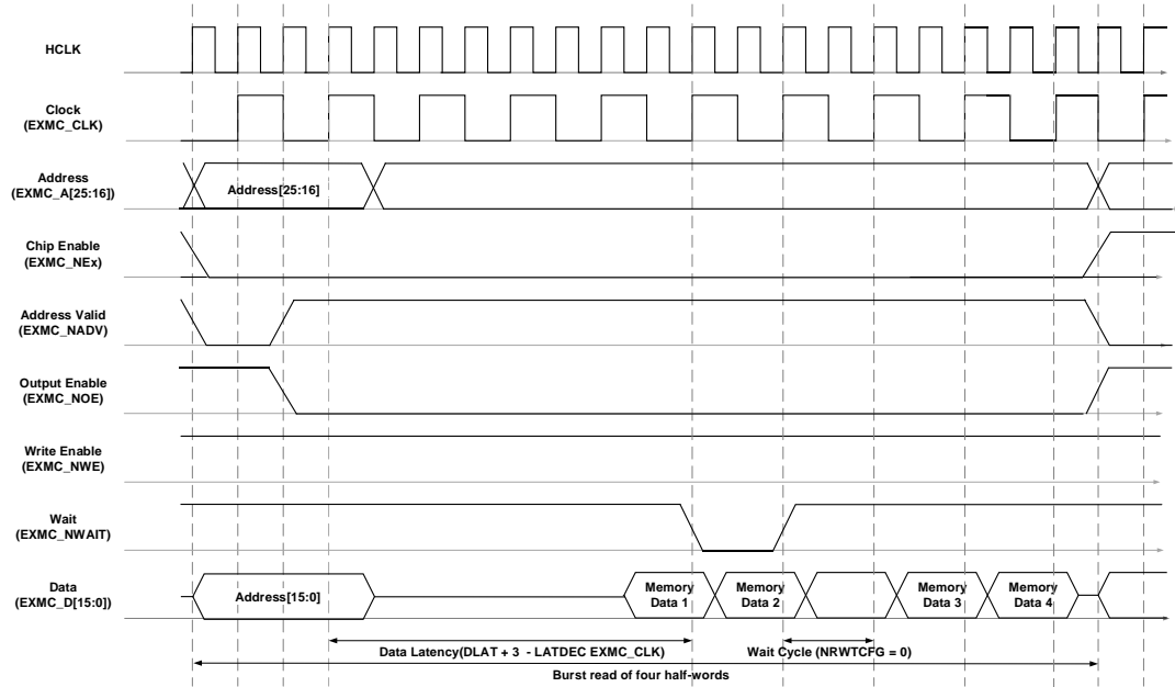
Figure 30-22. Read timing of synchronous multiplexed burst mode
