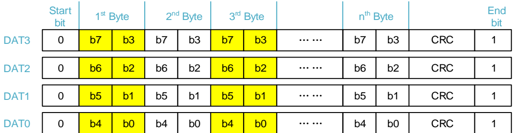
Figure 29-10. 4-bit data bus width
