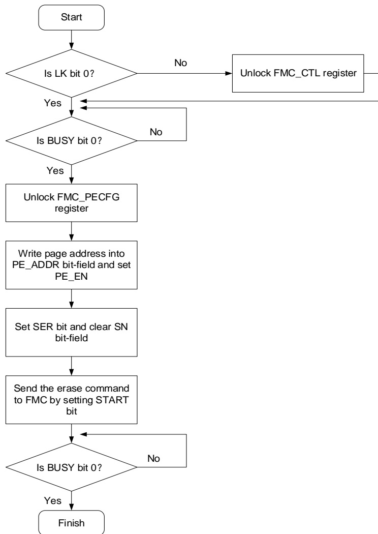
Figure 3-1. Process of page erase operation
