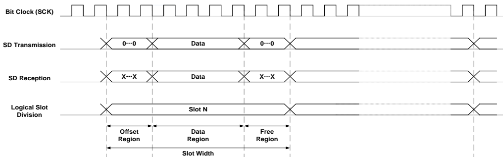
Figure 26-12 Data configuration
