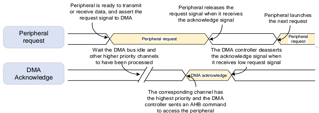
Figure 14-3. Handshake mechanism
