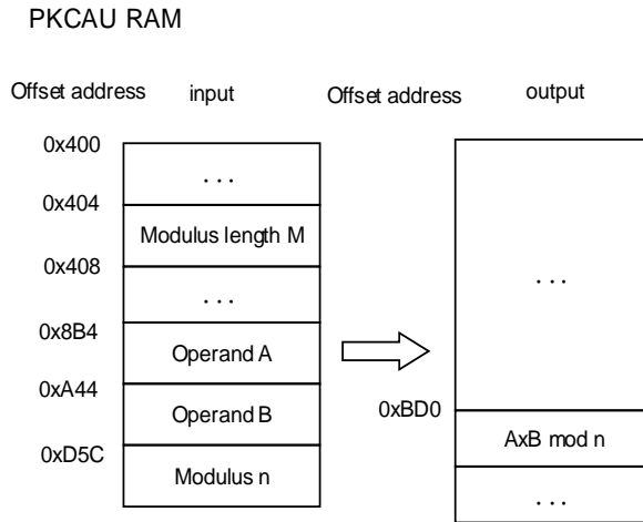
Figure 11-14. Montgomery multiplication
