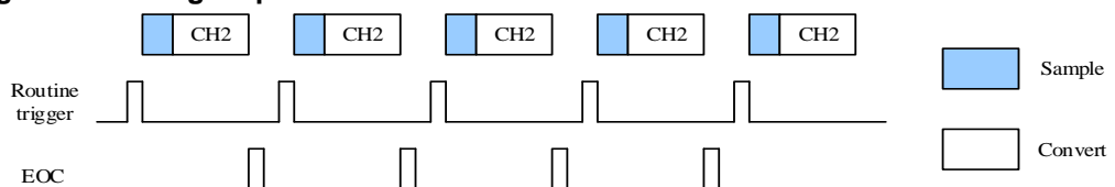
Figure 18-2. Single operation mode
