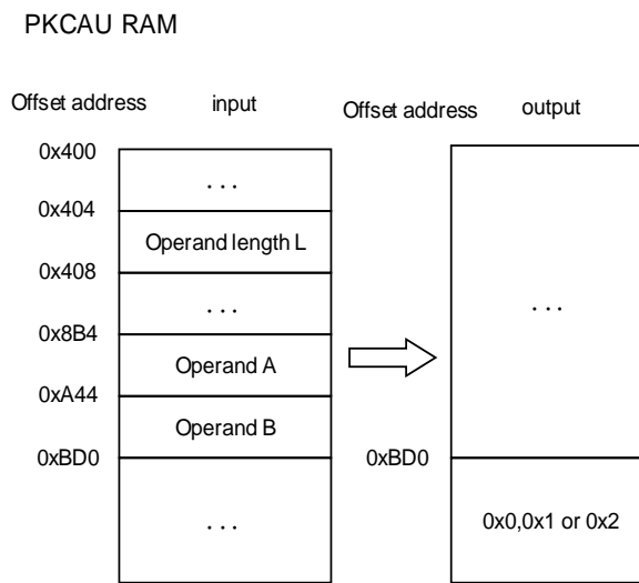
Figure 11-8. Arithmetic comparison
