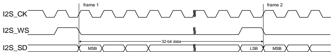
Figure 25-37. PCM standard short frame synchronization mode timing diagram (DTLEN=10, CHLEN=1, CKPL=1)
