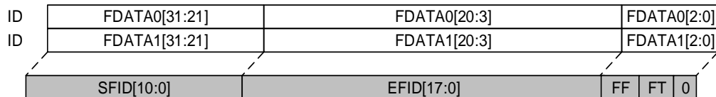
Figure 31-9. 32-bit list mode filter
