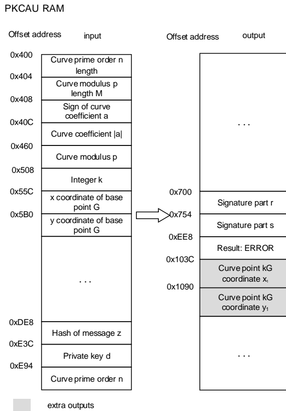
Figure 11-22. ECDSA sign
