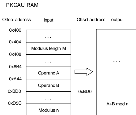
Figure 11-10. Modular addition
