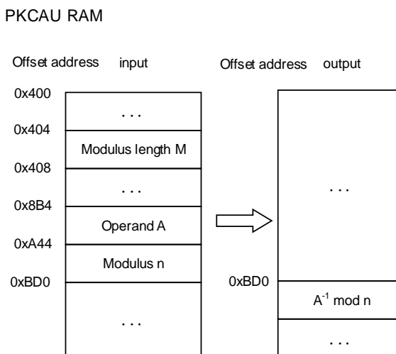
Figure 11-17. Modular inversion
