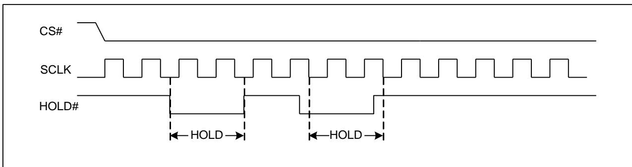
Figure 5-2. Hold Condition
